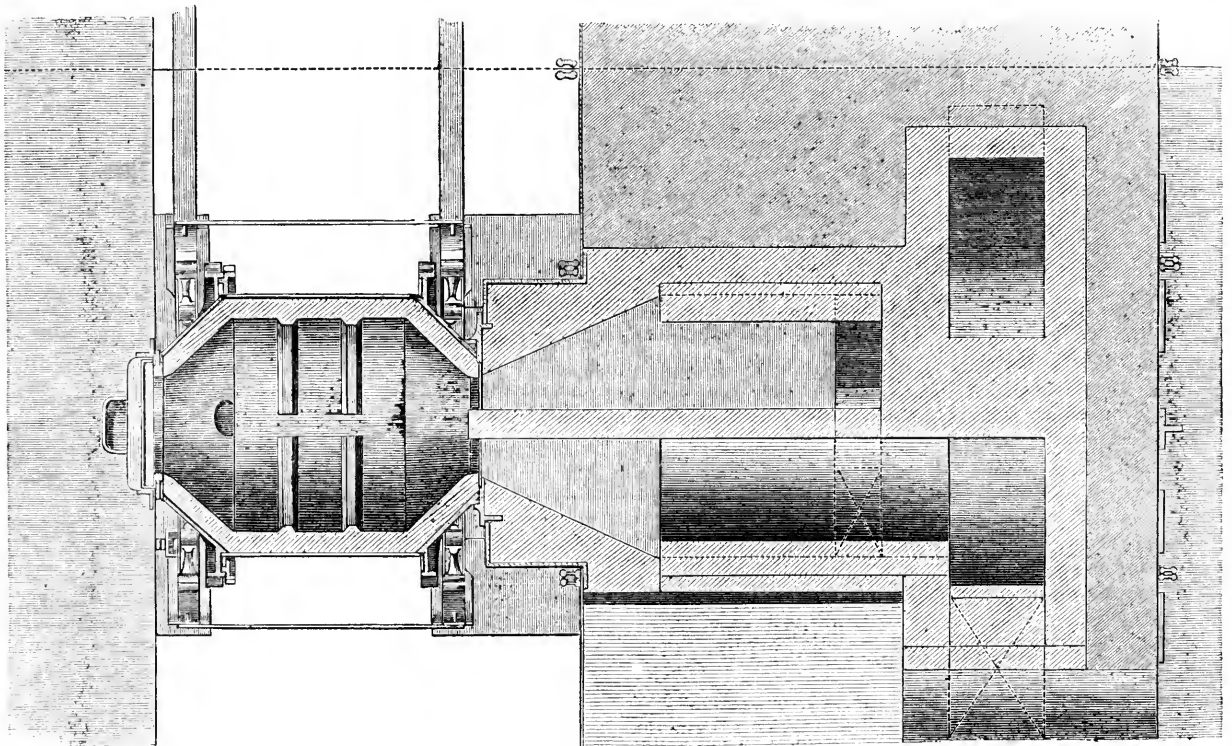
FIG. 58.—Siemens Rotator—Sectional Plan.
