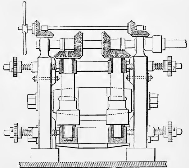
FIG 48.—Universal Rolls.
