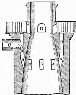
FIG. 27.—Collecting Top.
