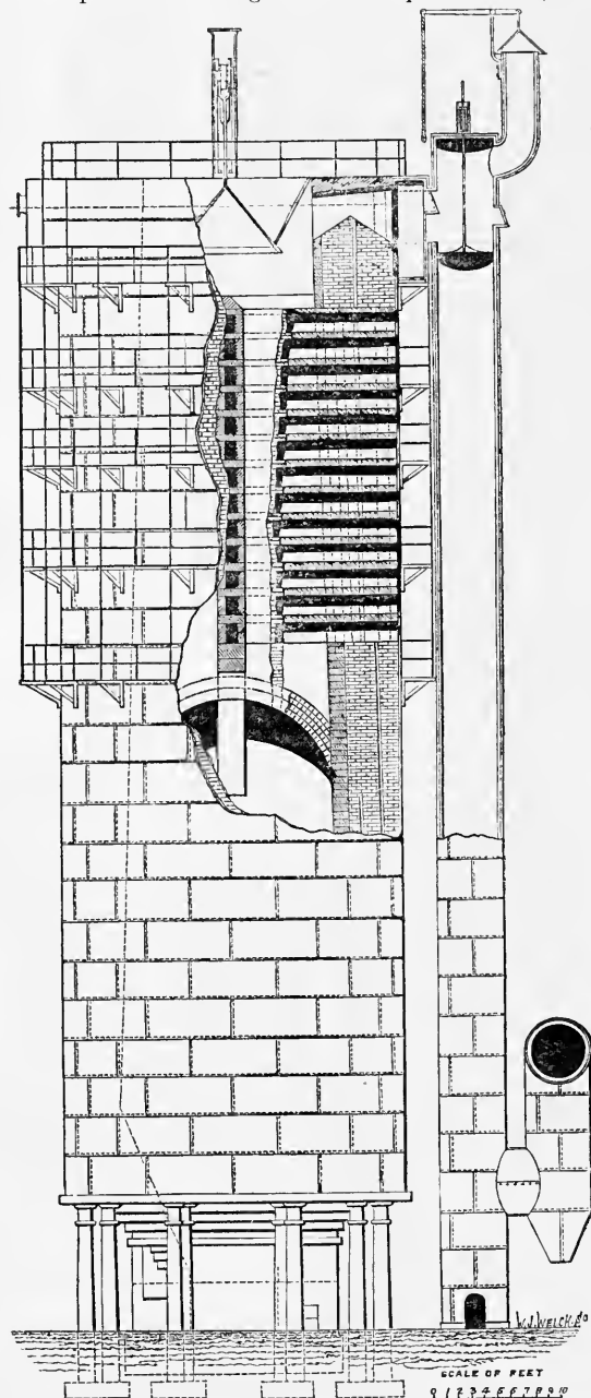
FIG. 13.—Ferrie's Furnace.
