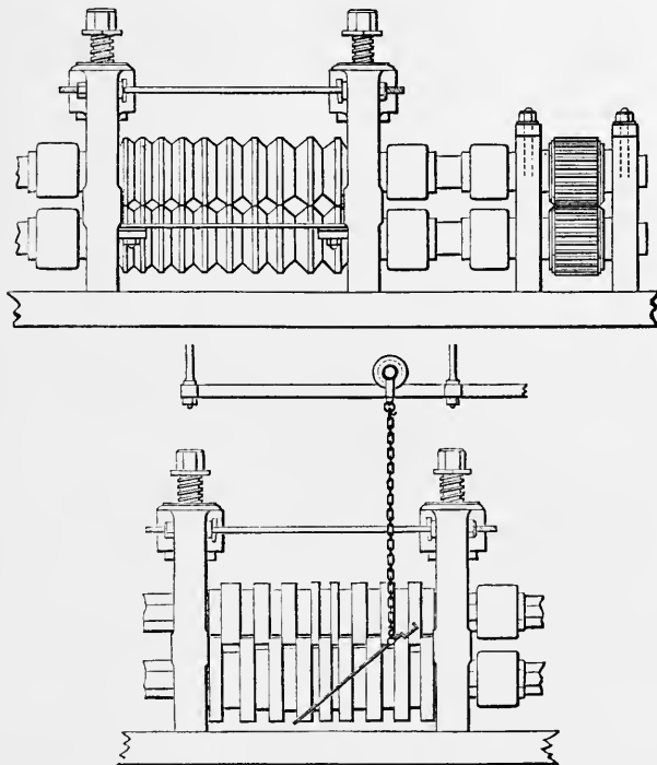
FIG. 46.—Two-high Trains.
