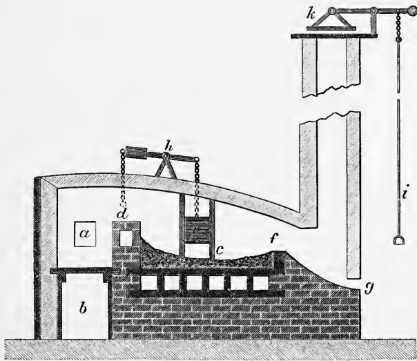
FIG. 32.—Puddling Furnace.
