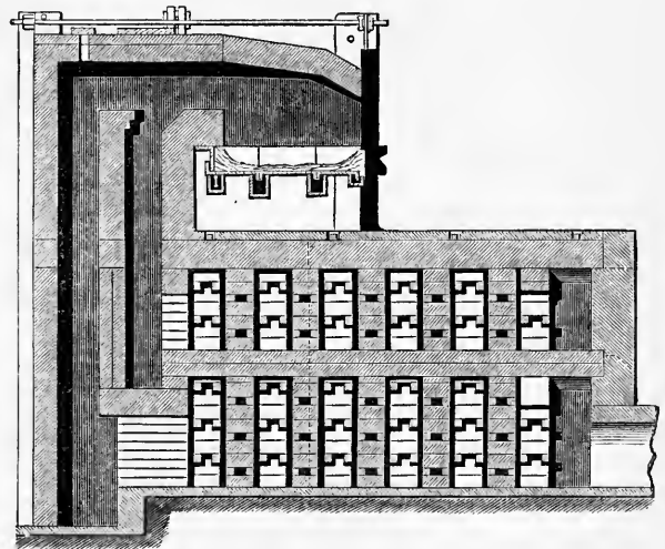
FIG. 33.—Siemens Regenerative Puddling Furnace.
