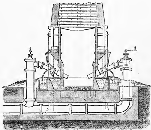
FIG. 30.—Refinery—Elevation.
