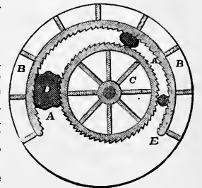
FIG. 43.—Revolving Squeezer.
