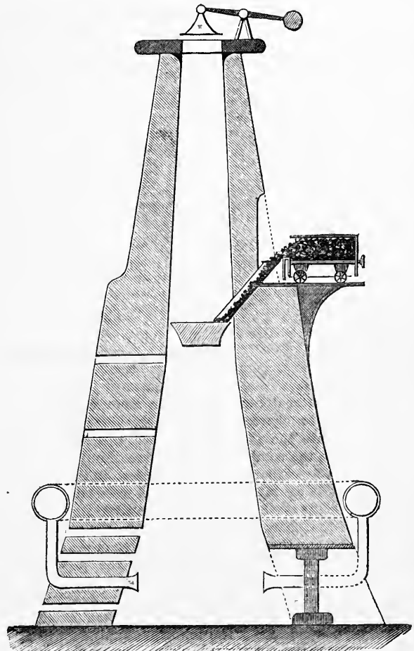
FIG. 2.—Westmann's Kiln.
