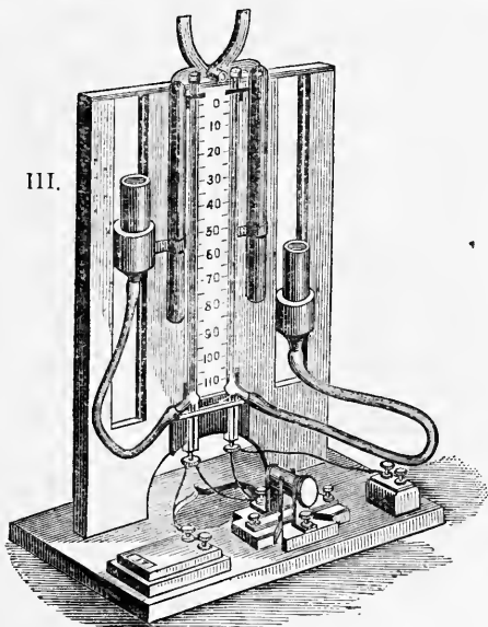
Fig. 22.—I. Siemens Electrical Pyrometer. II. Section of Heated End. III. Double Voltmeter.
