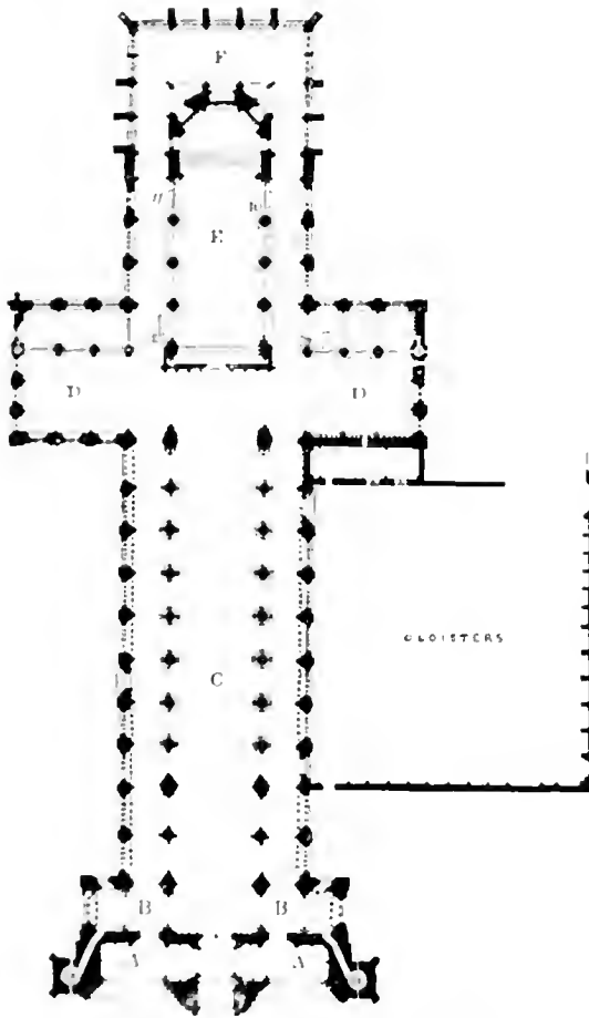
PLAN OF PETERBOROUGH CATHEDRAL (FROM STRAVER'S "HAND-BOOK.")
