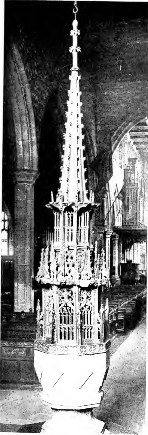
HALIFAX, YORKS., COUNTER-WEIGHTED
