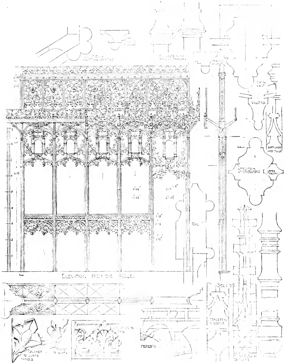
SOUTHWOLD, SUFFOLK, SCREEN BETWEEN QUIRE AND SOUTH AISLE
