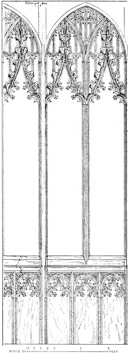
ADDLETHORPE, LINCS., TWO-LIGHT LINCOLN TYPE
