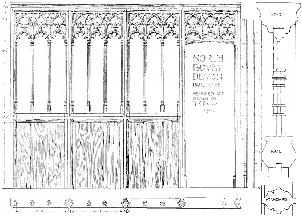
SQUARE PANEL SCREEN, DEVON TYPE, MID-FIFTEENTH CENTURY
