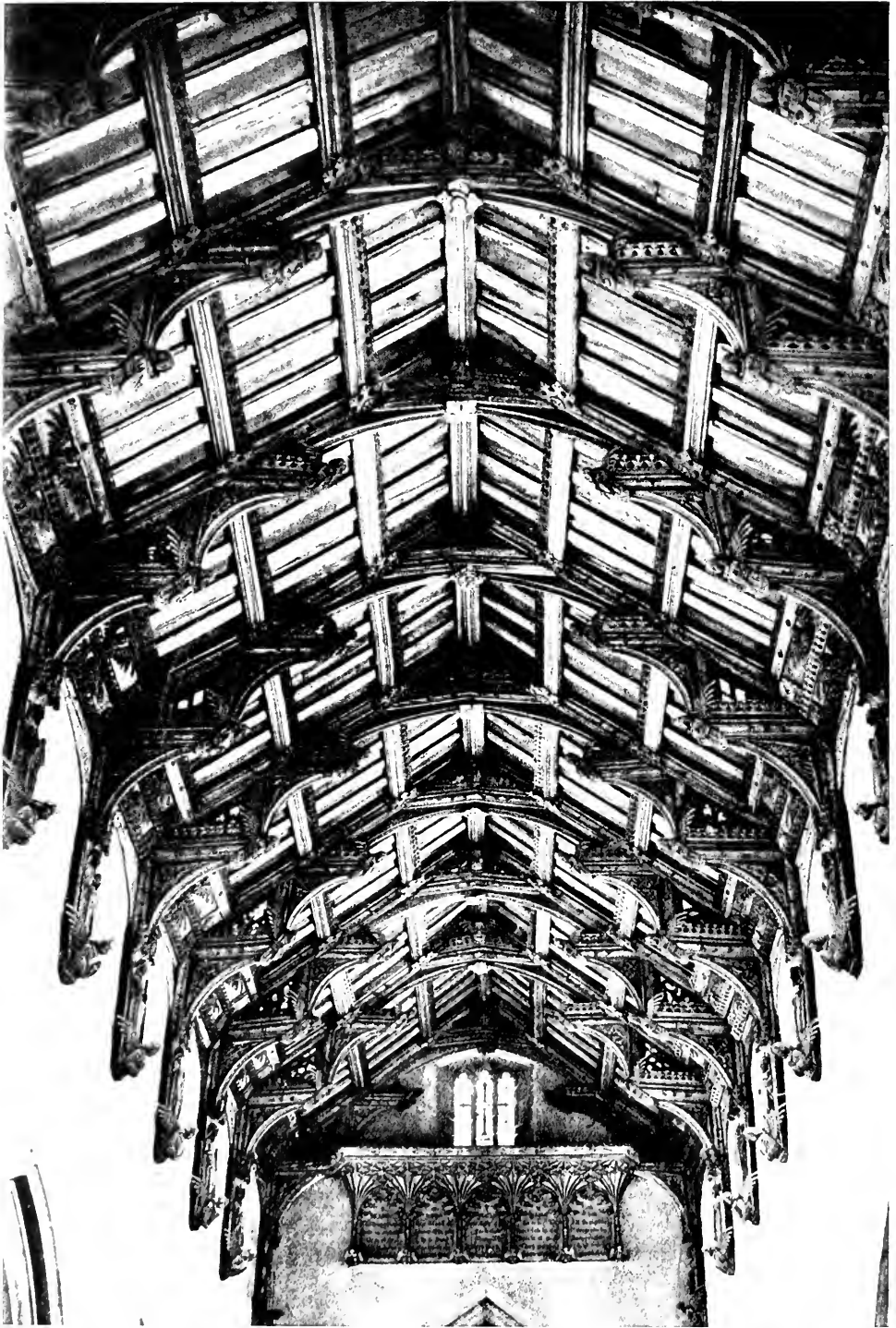
WOOLPT, SUFFOLK, "FALSE" DOUBLE HAMMER-BEAM ROOF
