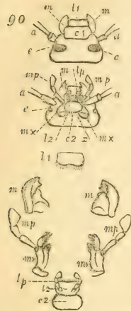
The different parts of the mouth of a beetle ( Blaps )— l1 , upper lip— m , mandibles— mx , maxillæ; mp , maxillary palpi; c2 , chin or mentum; l2 , labium; lp , labial palpi.
