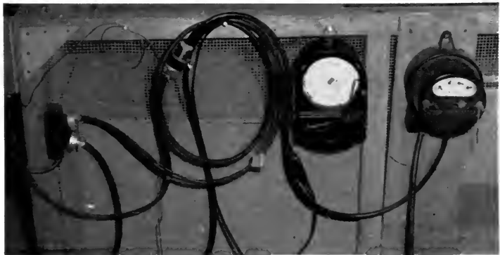
Tempscribe on-off recorder and watt-hour meter used in all tests. (Fig. 12)
