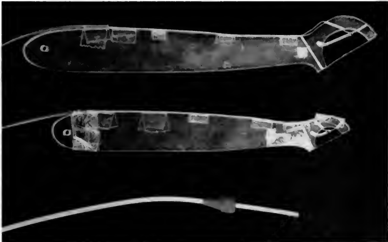
Thermocouple measuring instruments: (A) large plexiglass skin-temperature measuring instrument joining all seven strands of thermocouple wire; (B) small plexiglass skin-temperature measuring instrument joining only one strand of thermocouple wire; (C) rectal probe for measuring body temperature. (Fig. 10)
