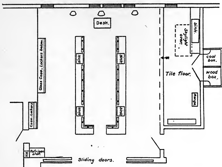
Fig. 5. School kitchen planned for 16 pupils, 27 x 34 feet
