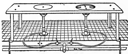
Fig. 24. Hot plate No. 1, used at Teachers College
