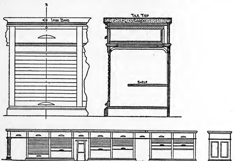
Fig. 17. Table with drawers and cupboards underneath
