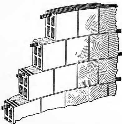
FIG. 122. Tile silo construction
