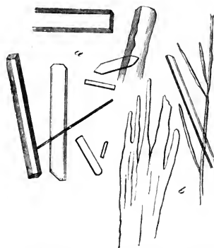
FIG. 43.—Crystals of urea: a , four-sided prisms; b , indefinite crystals, such as are usually formed from alcohol solutions.
