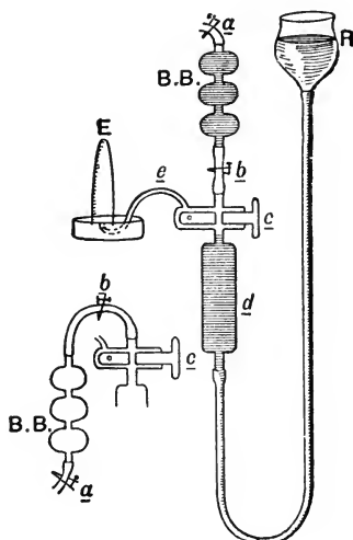
FIG. 80.—L. Hill's air-pump.
