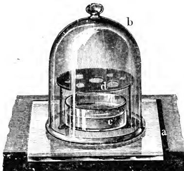
FIG. 62.—A desiccator. (Gscheidlen.) a, glass plate; b, bell-jar; c, dish of sulphuric acid; d, stand for capsules.
