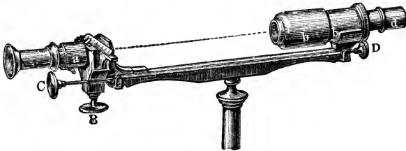
FIG. 74.—Soleil's saccharimeter.
