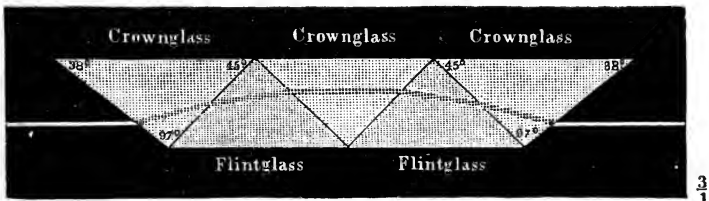
FIG. 34.—Arrangement of prisms in direct-vision spectroscopé.
