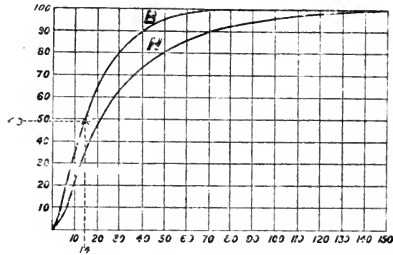
FIG. 39.—Dissociation of oxygen curves for blood (B) and hæmoglobin solution (H) at 38° C. The figures along the base line are pressures in millimetres of mercury, and those along the ordinate are percentages of oxygen. (Bohr.)
