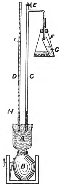
FIG. 40.—Barcroft's apparatus for obtaining the blood gases.
