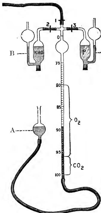
FIG. 81.—Waller's apparatus for gas analysis.
