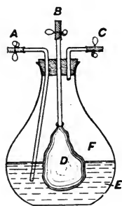
FIG. 38. Loewy's Aërotonometer.
