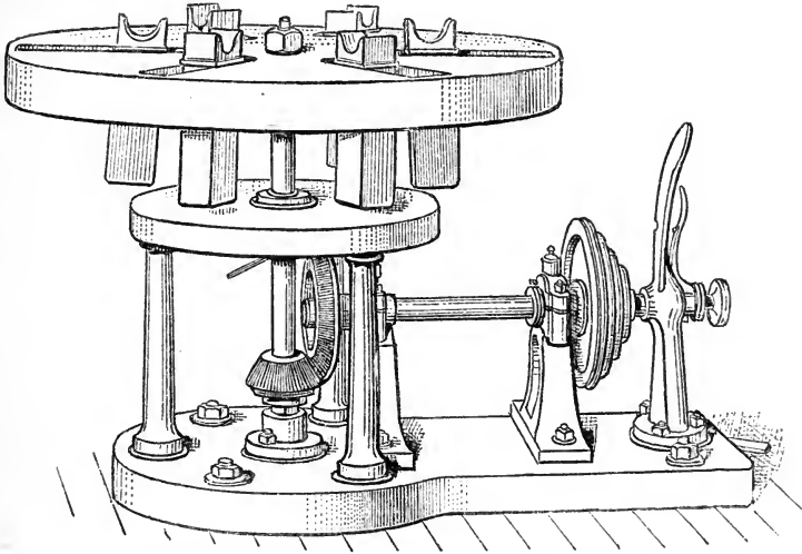
FIG. 60.—Centrifugal machine as made by Runne. Glass vessels containing the substances to be centrifugalised are placed within the six metallic tubes which hang vertically while the disc is at rest; when the machinery is set going they fly out into the horizontal position.
