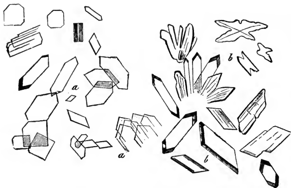
FIG. 44.— a , nitrate; b , oxalate of urea.
