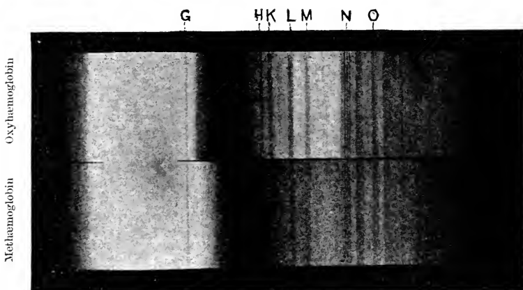
FIG. 59.—The photographic spectrum of oxyhæmoglobin and methæmoglobin. (Gamble.)
