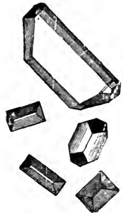
FIG. 45.—Ammonio-magnesium or triple phosphate.
