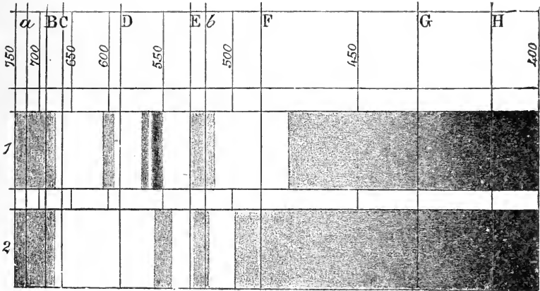
FIG. 61.—1, Absorption spectrum of myohaematin, as seen in muscle rendered transparent by glycerin. 2, Absorption spectrum of modified myohaematin.
