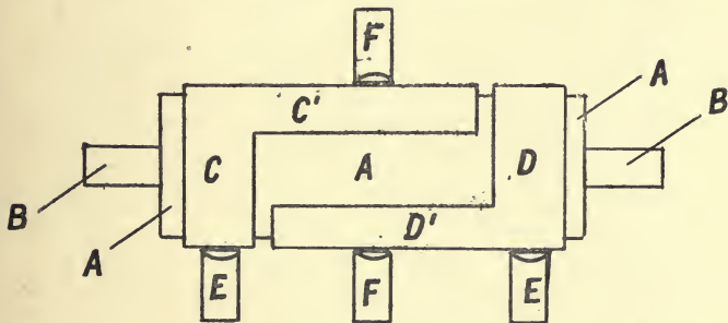
FIG. 7.—Ruhmkorff's Commutator
