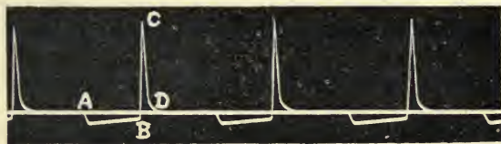
FIG. 14.—Graphic record of the secondary current from a well-designed coil.
