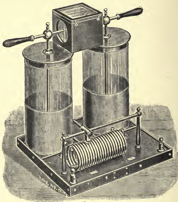
FIG. 44.—D'Arsonval's Transformer
