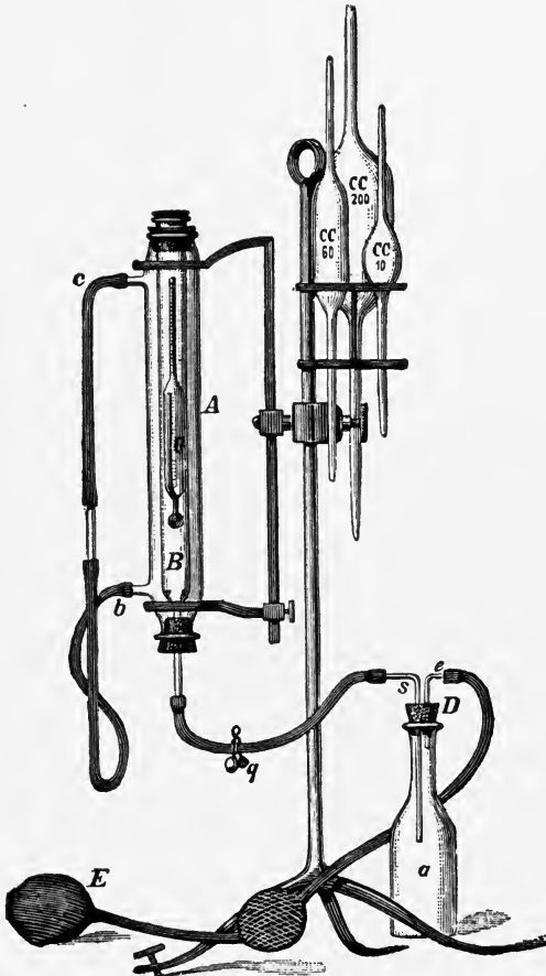
Soxhlet's apparatus for fat-determination.
