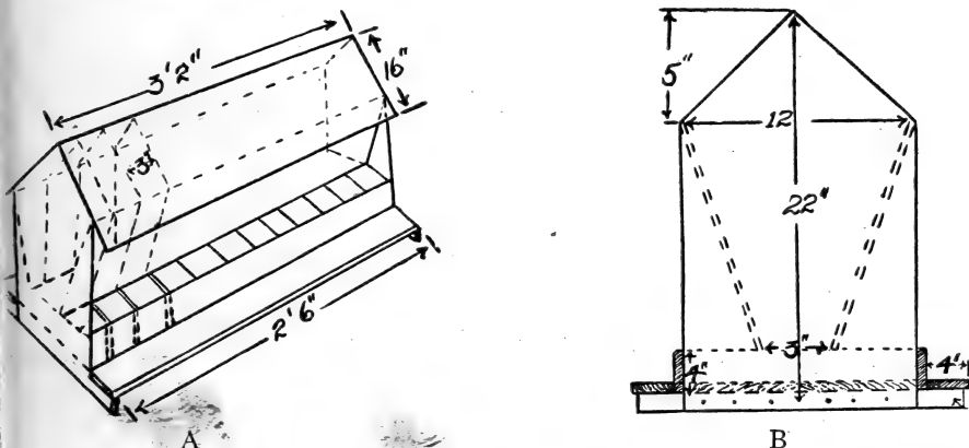
Fig. 34. A, angle view of an outdoor mash hopper. B, end diagram of same. This mash hopper is provided with three small compartments one for grit, one for charcoal, and one for crushed oyster shell. The large compartment is for dry mash.
