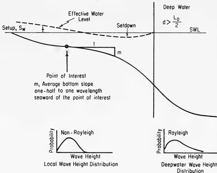
Figure 2. Definition sketch.
