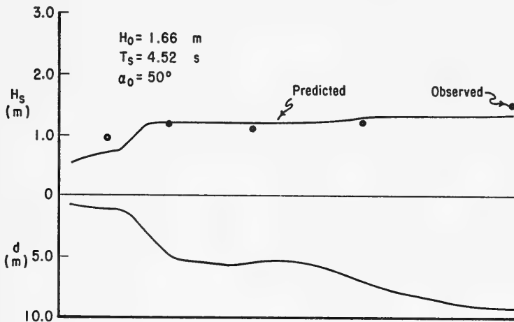
Figure 9. Observed and predicted wave height at the PRF, 13 September 1978.
