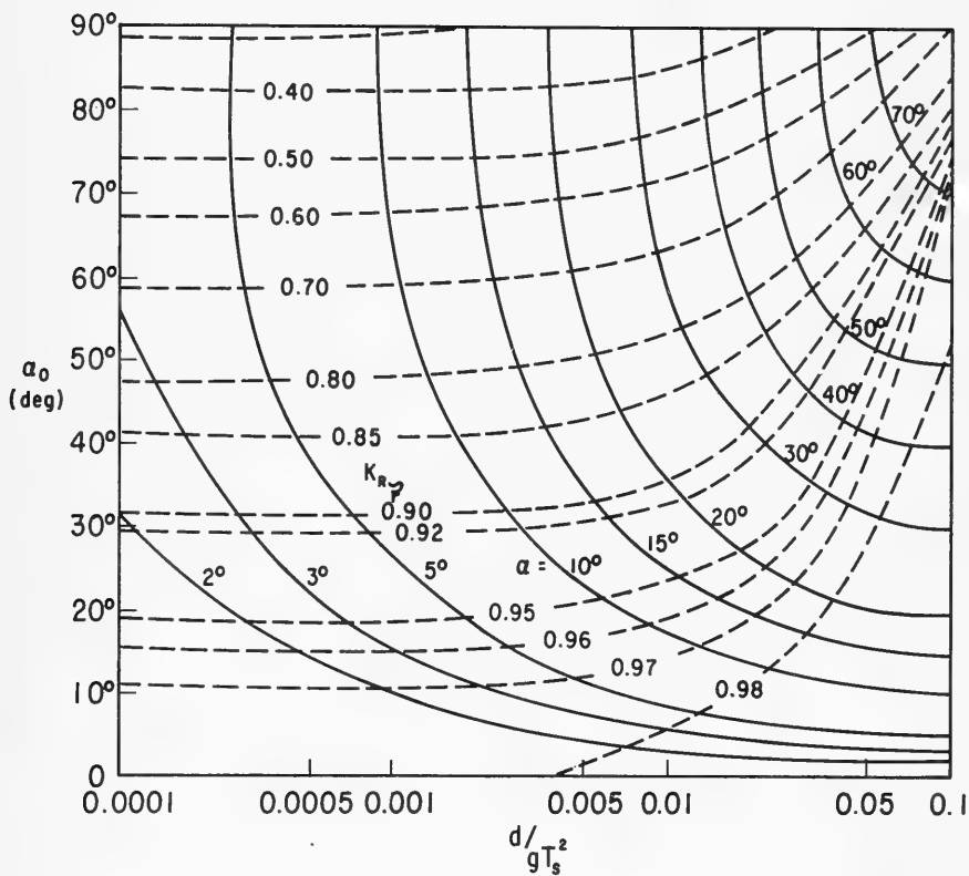
Figure A-3. Wave refraction for S^* = 37 .
