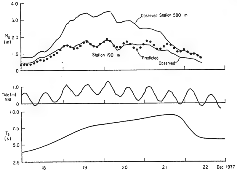
Figure 6. Observed and predicted wave conditions at the FRF 18 to 22 December 1977.
