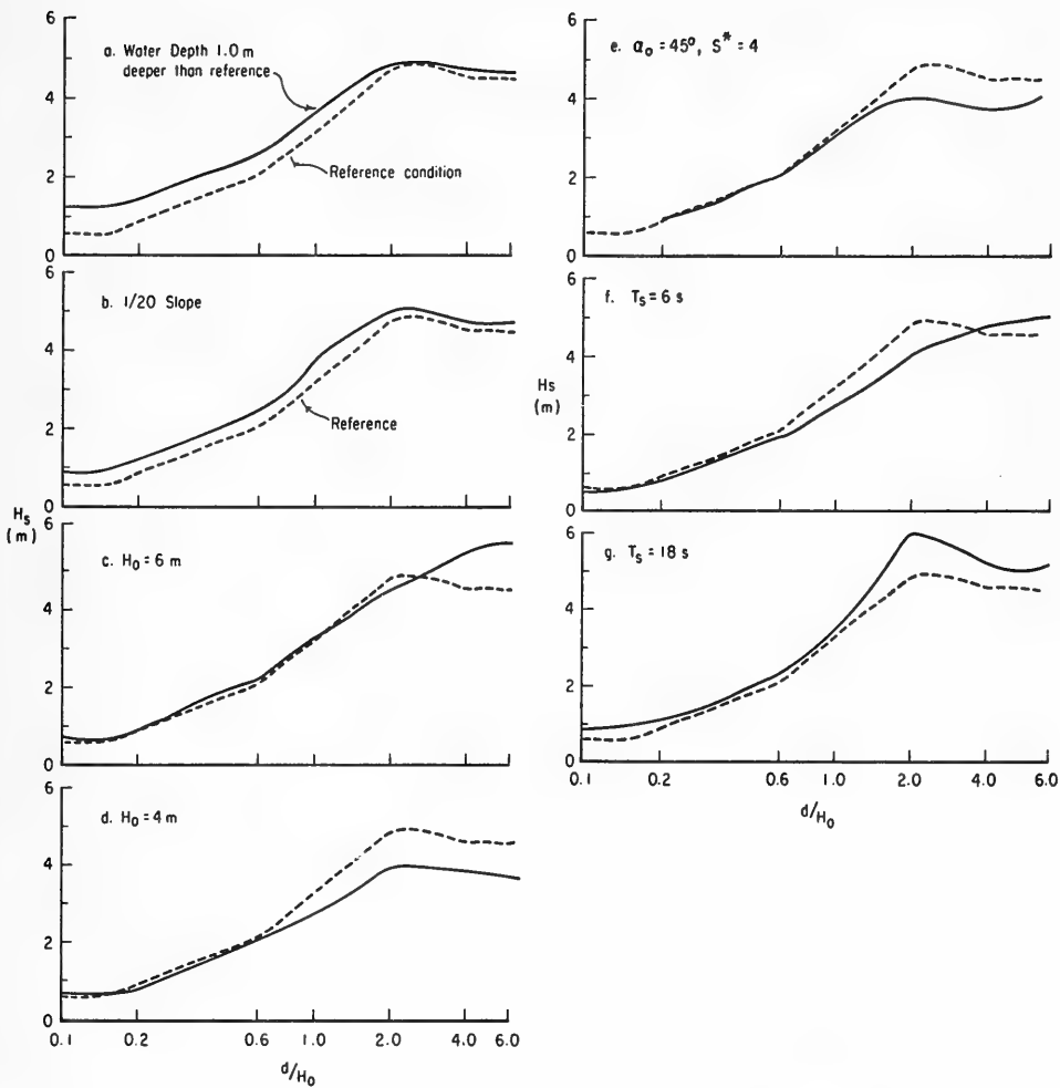
Figure 3. Sensitivity analysis of nearshore predicted significant wave heights.
