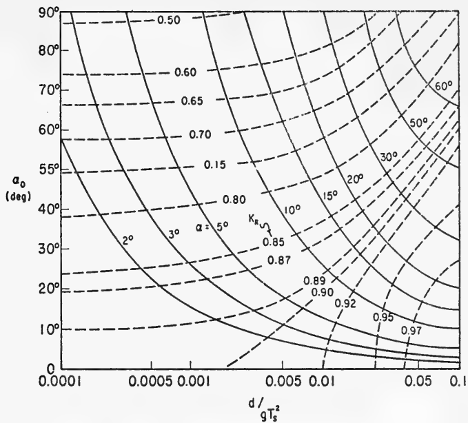
Figure A-1. Wave refraction for S^* = 4 .
