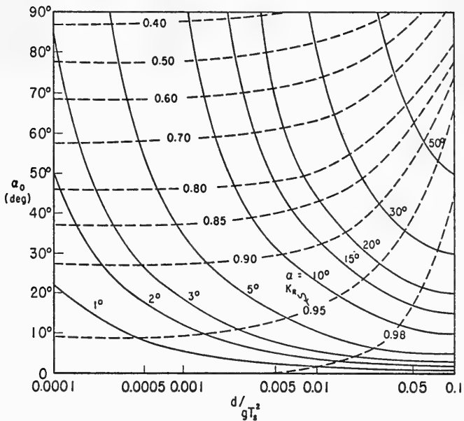
Figure A-2. Wave refraction for S^* = 12 .
