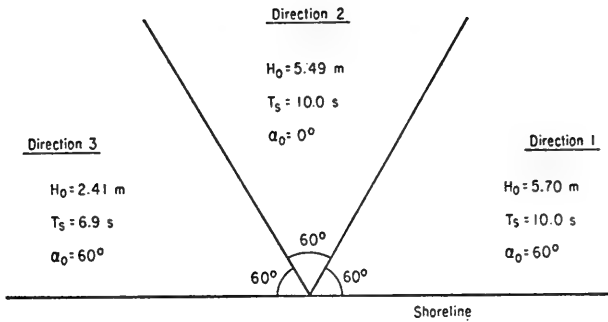
Figure 10. Deepwater wave conditions.
