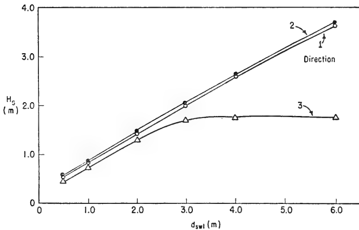
Figure 11. Predicted nearshore wave height.
