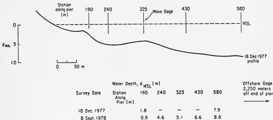
Figure 4. Profile at the Field Research Facility.
