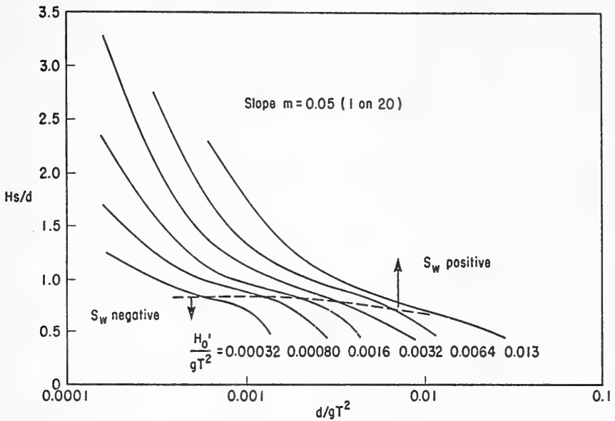
Figure C-3. Nearshore significant wave height diagram for a 1/20 beach slope.
