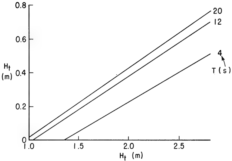
b. Predicted transmitted wave heights.
