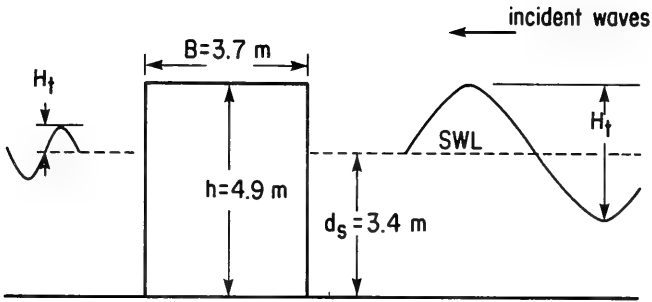
a. Profile view of conditions for Example 2.
