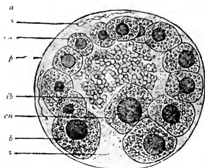
FIG. 64.—Blastula of the opossom ( Didelphys ). (From Selenka.) a animal pole of the blastula, v vegetal pole, en mother-cell of the entoderm, ex ectodermic cells, s spermia, ib unucleated yolk-balls (remainder of the food-yolk), p albumin membrane.
