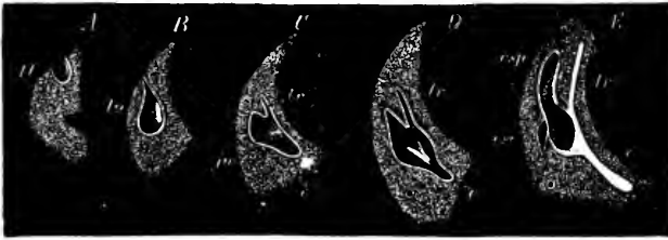
FIG. 322.—Development of the auscultory labyrinth of the chick, in five successive stages ( A-E ). (Vertical transverse sections of the skull.) f auscultory pits, lv auscultory vesicles, lv labyrinthine appendage, c rudimentary cochlea, csb posterior canal, cse external canal, jv jugular vein. (From Reissner.)
