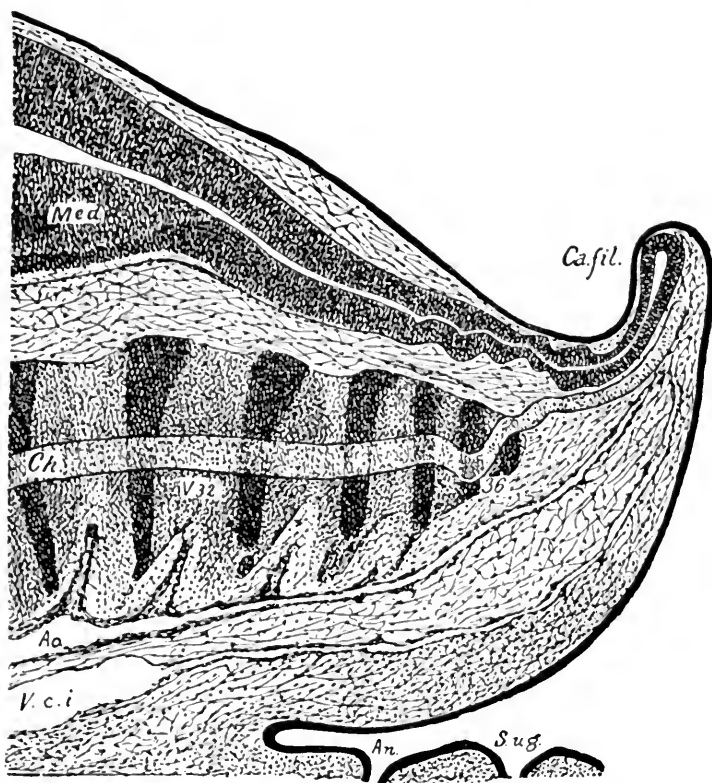
FIG. 182.—Median longitudinal section of the tail of a human embryo, two-thirds of an inch long. (From Ross Granville Harrison.) Med medullary tube, Ca.fil. caudal filament, ch chorda, ao caudal artery, V.c.i caudal vein, an anus, Sug. sinus urogenitalis.
