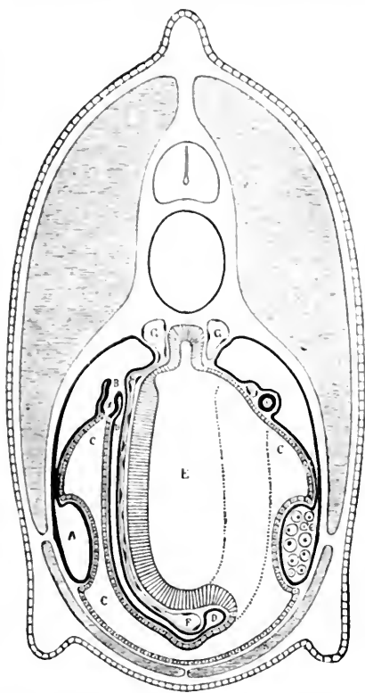
FIG. 217.—Transverse section through the middle of the Amphioxus. (From Boveri.) On the left a gill-rod has been struck, and on the right a gill-cleft; consequently on the left we see the whole of a proneural canal ( x ), on the right only the section of its fore-leg. A genital chamber (ventral section of the gonocoel), x pronephridium, B its coelom-aperture, C atrium, D body-cavity, E visceral cavity, F subintestinal vein, G aorta (the left branch connected by a branchial vessel with the subintestinal vein), H renal vessel.
