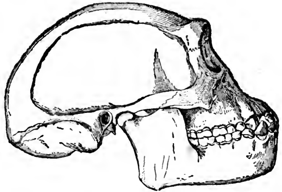
FIG. 283.—Skull of the fossil ape-man of Java ( Pithecanthropus erectus ), restored by Eugen Dubois.
