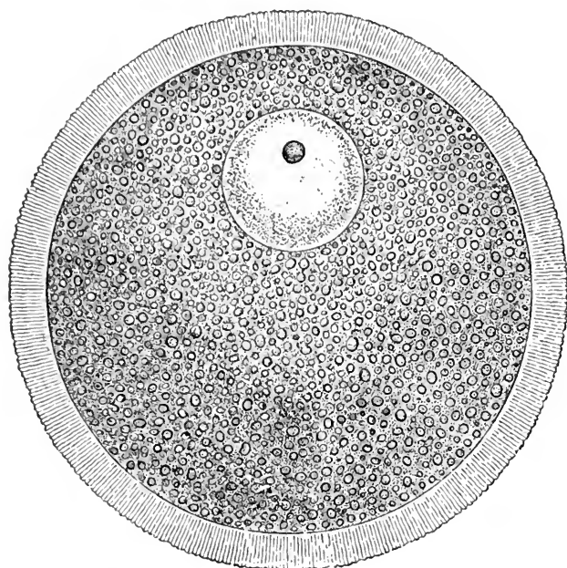
FIG. 14.—The human ovum, taken from the female ovary, magnified 500 times. The whole ovum is a simple round cell. The chief part of the globular mass is formed by the nuclear yolk ( deutoplasm ), which is evenly distributed in the active protoplasm, and consists of numbers of fine yolk-granules. In the upper part of the yolk is the transparent round germinal vesicle, which corresponds to the nucleus . This encloses a darker granule, the germinal spot , which shows a nucleolus . The globular yolk is surrounded by the thick transparent germinal membrane ( ovolemma , or zona pellucida ). This is traversed by numbers of lines as fine as hairs, which are directed radially towards the centre of the ovum. These are called the pore-canalals; it is through these that the moving spermatozoa penetrate into the yolk at impregnation.
