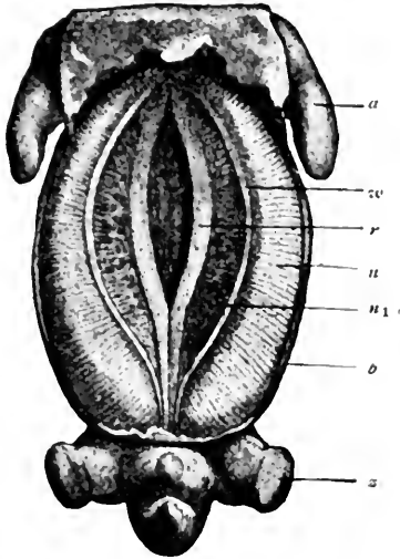
FIG. 388.—Pig-embryo, three-fifths of an inch long, magnified six times, seen from the ventral side. a fore leg, z hind leg, v ventral wall, r sexual prominence, n nephroduct, n primitive kidneys, n 1 their inner part. (From Oscar Schultze .)
