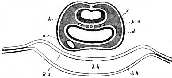
FIG. 381.—Transverse section of the head of a chick-embryo, thirty-six hours old. Underneath the medullary tube the two primitive aortas ( pa ) can be seen in the head-plates ( s ) at each side of the chorda. Underneath the gullet ( d ) we see the aorta-end of the heart ( ae ), hh cervical cavity or head-cœlom, hh top of heart, ks head-sheath, amniotic fold, h horny plate. (From Remak .)
