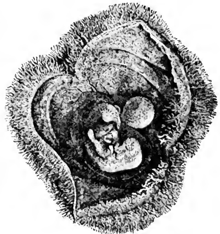
FIG. 193.—Human embryo of the fourth week, with its membranes, like Fig. 205, but a little older. The yolk-sac is rather smaller, the amnion and chorion larger
