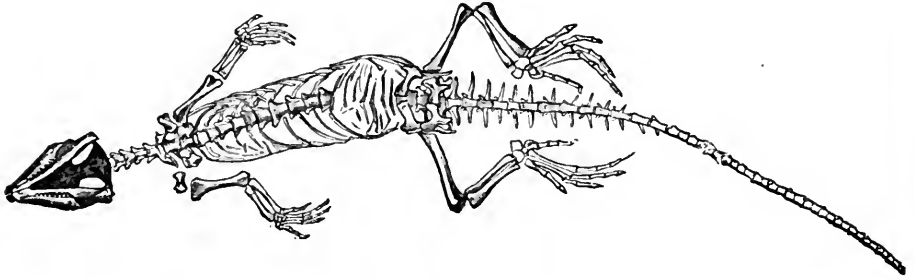
FIG. 265.— Homœosaurus pulchellus , a Jurassic proreptile from Kehlheim. (From Zittel.)
