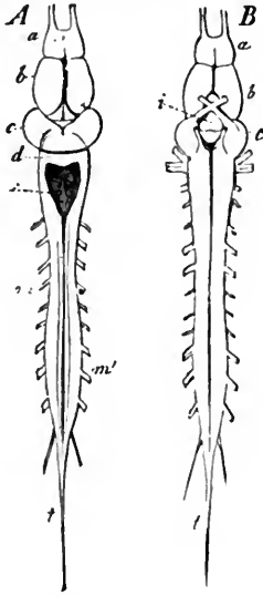
FIG. 300.—Brain and spinal cord of the frog. A from the dorsal, B from the ventral side. a olfactory lobes before the ( b ) fore brain, i infundibulum at the base of the intermediate brain, c middle brain, d hind brain, s quadrangular pit in the after brain, m spinal cord (very short in the frog); m' roots of the spinal nerves, t terminal fibres of the spinal cord. (From Gegenbaur.)
