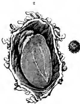
FIG. 186.—Human ovum of twelve to thirteen days (?). (From Allen Thomson.) 1. Not opened, natural size. 2. Opened and magnified. Within the outer chorion the tiny curved fetus lies on the large embryonic vesicle, to the left above.
