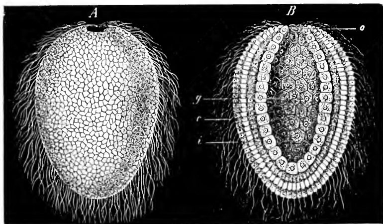
FIG. 36.—Gastrula of a lower sponge ( olyntus ). A external view, B longitudinal section through the axis, g primitive-gut cavity, o primitive mouth-aperture, i inner cell-layer (entoderm, endoblast, gut-layer), e external cell-layer (outer germinal layer, ectoderm, ectoblast, or skin-layer).
