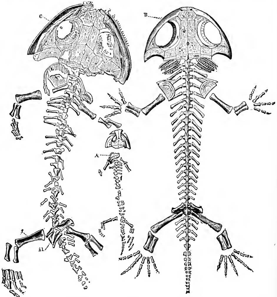
FIG. 260.—Fossil amphibian from the Permian, found in the Plauen terrain near Dresden ( Branchiosaurus amblystomus ). (From Credner.) A skeleton of a young larva. B larva, restored, with gills. C the adult form, natural size.
