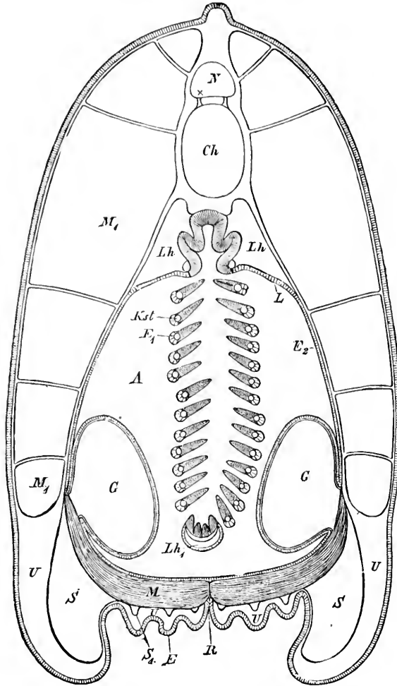
FIG. 216.—Transverse section of the lancelet, in the fore half. (From Ralph .) The outer covering is the simple cell-layer of the epidermis ( E ). Under this is the thin corium, the subcutaneous tissue of which is thickened; it sends connective-tissue partitions between the muscles ( M 1 ) and to the chorda-sheath. N medullary tube, Ch chorda, Lh body-cavity, A atrium, L upper wall of same, E 1 inner wall, E 2 outer wall, Lh 1 ventral remnant of same, Kst gill-rods, M ventral muscles, R seam of the joining of the ventral folds (gill-covers), G sexual glands.
