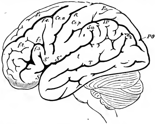
FIG. 203.—The human brain, seen from the left. (From H. Meyer .) The furrows of the cerebrum are indicated by thick, and those of the cerebellum by finer lines. Under the latter we can see the medulla oblongata. f_1 - f_2 frontal convolutions, C central convolutions, S fissure of Sylvius, T temporal furrow, Pa parietal lobes, A_1 angular gyrus, P_0 parieto-occipital fissure.
