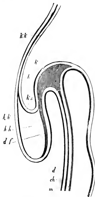
FIG. 148.—Longitudinal section of the fore half of a chick-embryo at the end of the first day of incubation (seen from the left side). k head-plates, ch chorda. Above it is the blind fore-end of the ventral tube ( m ); below it the capital cavity of the gut. d gut-gland layer, df gut-fibre layer, h horn plate, hh cavity of the heart, hk heart-capsule, ks heart-sheath, kk head-capsule. (From Remak.)
