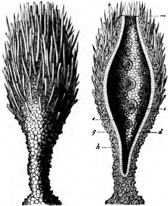
FIGS. 234 and 235.— Prophysema prlmordiale , a living gastræad. Fig. 234. The whole of the spindle-shaped animal (attached below to the floor of the sea). Fig. 235. The same in longitudinal section. The primitive gut ( d ) opens above at the primitive mouth ( m ). Between the ciliated cells ( g ) are the amœboid ova ( e ). The skin-layer ( h ) is encrusted with grains of sand below and sponge-spicules above.
