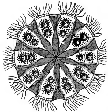
FIG. 232.—Section of same, showing how the pear-shaped cells in the centre of the gelatinous ball are connected by a fibrous process. Each cell has a contractile vacuole as well as a nucleus.
