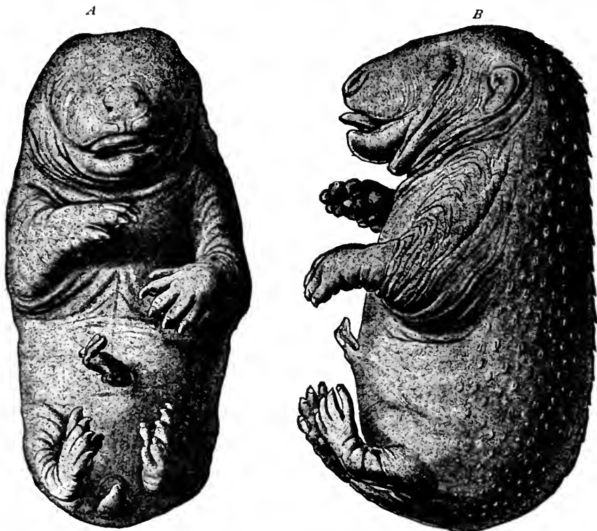
Fig. 289.—Embryo of a bear ( Ursus arctos ), twice natural size. A seen from ventral side, B from the left.
