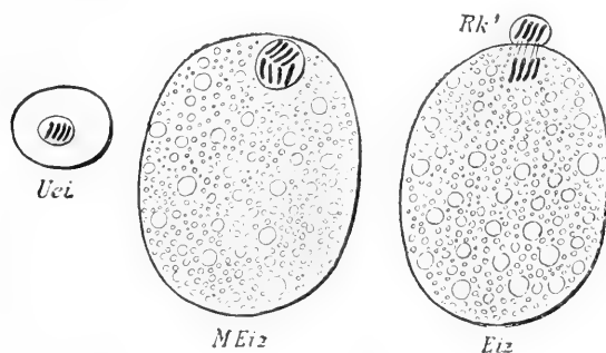
FIG. 78. Diagram of the maturation of a parthenogenetic ovum. The number of chromosomes normal to the species has been assumed to be four. Uei , a primitive germ-cell. MEi2 , a mother-egg-cell, with twice the normal number of chromosomes. Eiz , mature ovum after the separation of the first and only polar body. Rk' .
