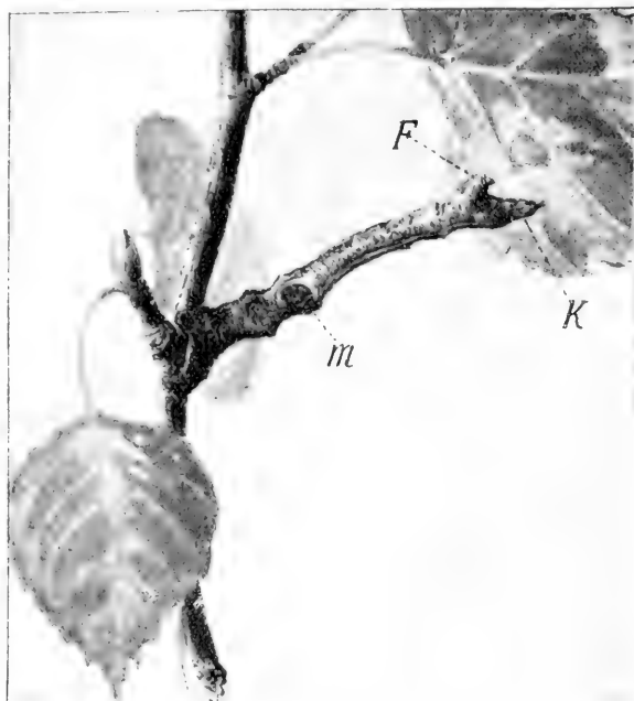
FIG. 17. Caterpillar of Selenia tetralnaria , seated on a birch twig. K , head. F , feet. m , tubercle, resembling a 'sleeping bud'; nat. size.
