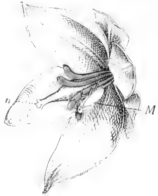
FIG. 51. The Yucca-moth ( Pro-miba yuccasella ). M , laying eggs in the ovary of the Yucca flower. n , the stigma. After Riley.
