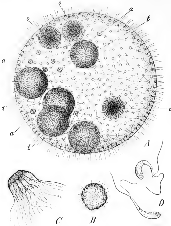
FIG. 63. Volvox aureus , after Klein and Schenck. A , besides the small flagellate somatic cells of the colony there are five large egg-cells ( t ) which are capable of parthenogenetic development, three recently fertilized egg-cells ( o ) and a number of male germ-cells ( a ) in process of multiplication. From each of these, by continued division, a bundle of spermatozoa arises. B , a bundle of thirty-two sperm-cells in process of development, seen from above. C , the same seen from the side. Magnified 687 times. D , individual spermatozoa, magnified 824 times.
