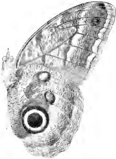
FIG. 6. Under surface of the wings of Culigo .
