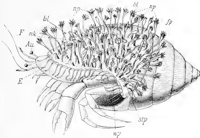
FIG. 34. Hermit-crab ( E ), within a Gasteropod shell, on which a colony of Podocoryne carneæ has established itself. From the common root-work (which is not clearly shown) there arise numerous nutritive polyps with tentacles ( np ), among which are smaller 'blastostyle' polyps with a circle of medusoid buds ( mk ), spine-like personæ ( stp ), and on the margin of the mollusc shell a row of defensive individuals ( wp ). F , antennæ. Au , eyes of the hermit-crab; slightly enlarged.
