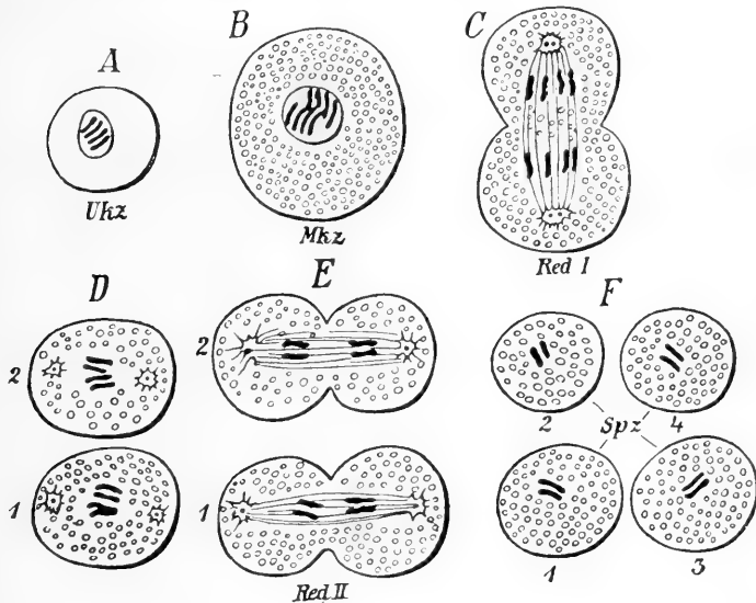
FIG. 77. Diagram of the maturation-divisions of the sperm-cell, adapted from O. Hertwig. A , primitive sperm-cell. B , mother-sperm-cell. C , first maturation division. D 1 and 2, the two daughter-cells. E , the second maturation division, by which the four cells of F arise, each with half the number of chromosomes.
