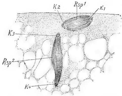
FIG. 79. The two maturation divisions of the 'drone eggs' (unfertilized eggs) of the Bee, after Petrunkevitch. Rsp 1 , the first directive spindle. k 1 and k 2 , the two daughter-nuclei of the same. Rsp 2 , the second directive spindle. k 3 and k 4 , the two daughter-nuclei. In the next stage k 2 and k 3 unite to form the primitive sex-nucleus. Highly magnified.
