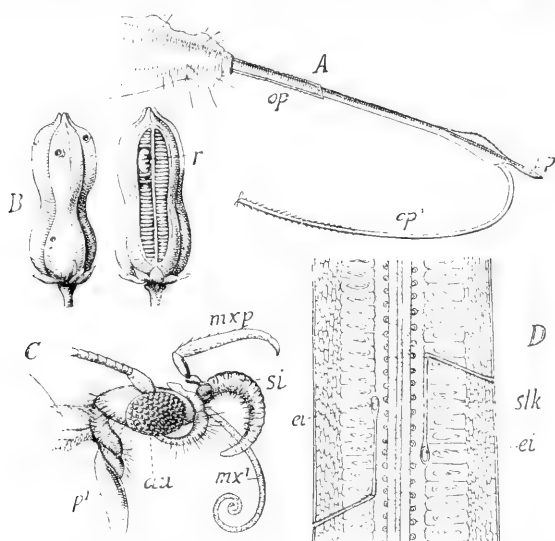
FIG. 52. The fertilization of the Yucca . A , ovipositor of the Yucca -moth. op , its sheath. sp , its apex. op' , the protruded oviduct. B , two ovaries of the Yucca , showing the holes by which the young moths escape, and ( r ) a caterpillar in the interior. C , head of the female moth, with the sickle-shaped process ( si ) on the maxillary palps for sweeping off the pollen and rolling it into a ball. mx' , the proboscis. au , eye. p' , base of first leg. D , longitudinal section through an ovary of the Yucca , soon after the laying of two eggs ( ei ). slk , the canal made by the ovipositor.
