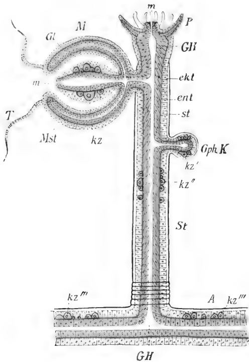
FIG. 94. Diagram to illustrate the phylogenetic shifting back of the origins of the germ-cells in medusoids and hydroids. A composite picture. A , branch of a polyp colony. P , polyp-head with mouth ( m ) and tentacles. St , stalk of the polyp. M , medusoid-bud with the bell ( Gl ). T , marginal tentacles. m , mouth. Mst , manubrium. GphK , a gonophore-bud. GH , gastric cavity. ekt , ectoderm. ent , endoderm. st , supporting lamella. The germ-cells ( kz ) arise in the medusoid in the ectoderm of the manubrium—first phyletic stage—where they also attain maturity. In the gonophore-bud ( GphK ) they arise in the ectoderm ( kz' ), or further down in the stalk of the polyp at kz'' —third phyletic stage, or in the ectoderm of the branch from which the polyp has arisen, at kz''' —fourth phyletic stage of the shunting of the originative area of the germ-cells. In the two last cases the germ-cells migrate until they reach their primitive place of origination in the medusoid, or in the corresponding layer of the medusoid gonophore, as may be more clearly seen in Fig. 95. Drawn from my sketch by Dr. Petrunkevitch.
