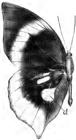
FIG. 55. Zeuroidia wallacei , male, showing four tufts of long, bristle-like, bright yellow scent-scales ( d ) on the upper surface of the posterior wing.
