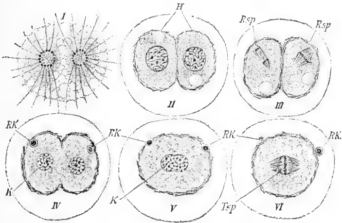
FIG. 84. Conjugation and polar body formation in the Sun-animalcule, Actinophrys sol , after Schaudinn. I , two free-swimming conjugated individuals, which in II have become surrounded by a transparent gelatinous cyst. III , formation of the directive spindles ( Rsp ). IV , the polar bodies are formed ( RK ); K , the two sex-nuclei. V , these are fused to form the conjugation-nucleus ( K ). VI , the conjugation-nucleus is transformed into the division-spindle; the polar bodies ( RK ) have penetrated the internal cyst-wall, and are in process of degeneration.
