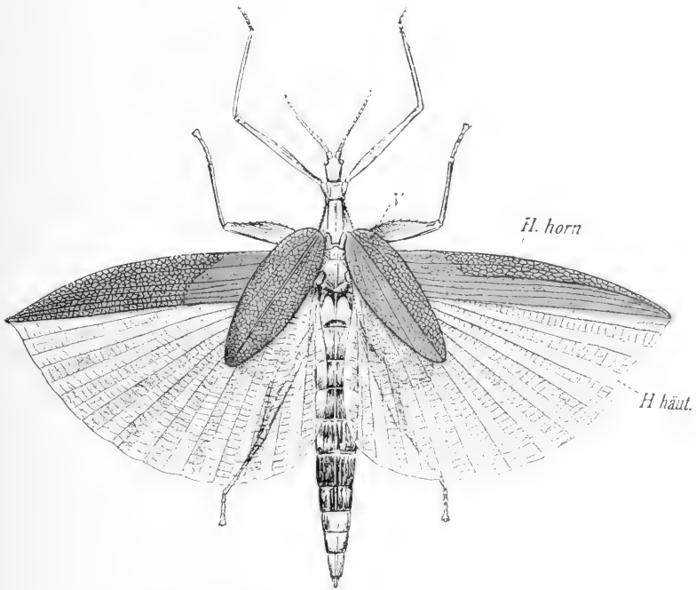
FIG. II. Tropidoderus childreni , after Brunner von Wattenwyl, in flying pose. V anterior wing. H. häut, membranous part of posterior wing. H. horn, horny portion.
