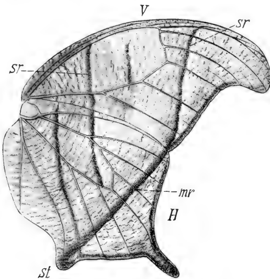
FIG. 15. Cerois chorineus , from the lower Amazon, in its resting attitude. V , anterior wing. H , posterior wing. mr , midrib of the apparent leaf. sr , lateral veins. st , hind of a leaf-stalk.
