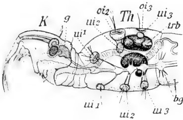
FIG. 89. Anterior region of the larva of a Midge ( Corethra plumicornis ). K , head. Th , thorax. ui , inferior imaginal disks. oi , superior imaginal disks. ui 1 , ui 2 , and ui 3 , the primordia of the limbs. oi 2 and oi 3 , the primordia of the wings and 'balancers.' g , brain. bg , chain of ventral ganglia with nerves which enter the imaginal disks. trb , tracheal vesicle. Enlarged about 15 times.
