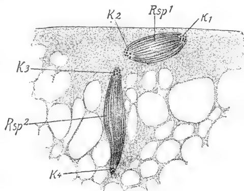
FIG. 79. The two maturation divisions in the unfertilized (drone-forming) egg of the bee, after Perrunkewitsch. Rsp 1 , first polar-body in division. K 1 and K 2 , the two daughter-nuclei thereof. Rsp 2 , second directive spindle. K 3 and K 4 , the two daughter-nuclei thereof. In the subsequent stage K 2 and K 3 unite to form the primordial sex-cell nucleus. Highly magnified.
