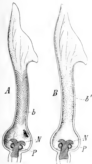
FIG. 43. Flower of Birthwort ( Aristolochia clematitis ) cut in half. A , before pollination by small flies. b , the bristles. B , after pollination. P , pollen mass. N , stigma. b , the bristles. b' , their remains. After H. Müller.
