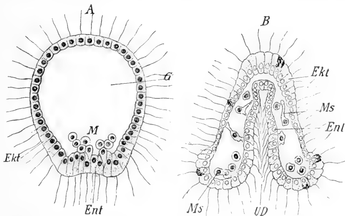
FIG. 92. Echinoderm-larva. A, blastula-stage; the primary mesoderm-cells ( M ) are being formed at the subsequent invagination-area of the endoderm ( Ent ). Ekt , the ectoderm. B, gastrula-stage; the archenteron ( UD ) has been invaginated ( Ent ), and between it and the ectoderm ( Ekt ) the mesoderm-cells ( Ms ) migrate into the gelatinous fluid which fills this cavity. There they attach themselves partly to the ectoderm, and partly to the endoderm. After Selenka.
