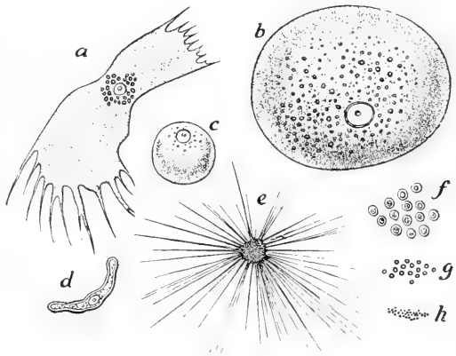
FIG. 66. Spermatozoa of various Daphnids. a , Sida . b , Bythotrephes . c , Daphnella . d , Moina paradoxa . e , Moina rectirostris . f , Eurycercus lamellatus . g , Alonella pygmaea . h , Peracantha truncata . All magnified 300 times.
