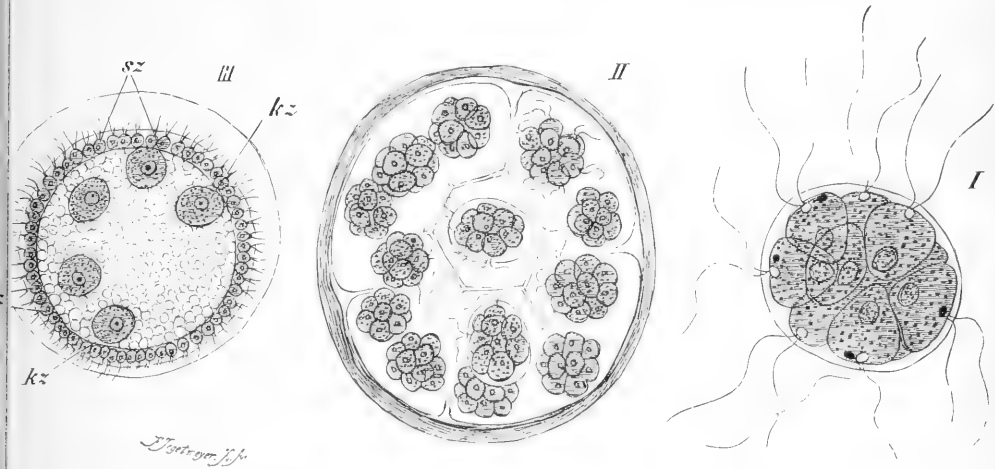
FIG. 62. Pandorina morum ; after Pringsheim. I, A young colony, consisting of 16 cells. II, Another colony, whose cells have reproduced daughter-colonies; all the cells uniformly alike. III, A young colony; sz , somatic cells; kz , germ-cells.
