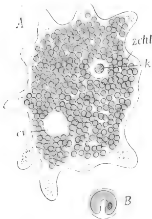
FIG. 36. A, Amöba viridis. k , the nucleus. cc , contractile vacuole. zchl , the zoochlorellæ. B , a single zoochlorella under high power. After A. Gruber.
