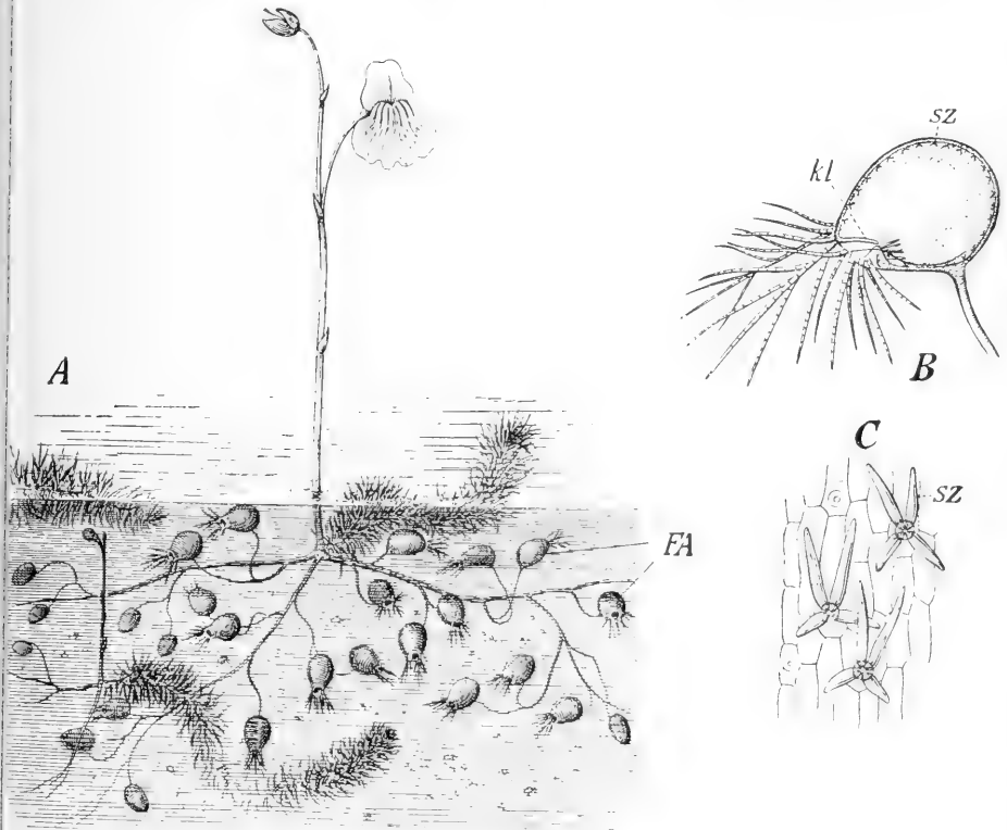
FIG. 23. Utricularia grafiiana , after Kerner. A, a plant in its natural position, floating in the water. FA, traps. B, a trap enlarged four times. sz, suctorial cells. kl, valve, which closes the entrance to the trap. C, suctorial cells on the internal wall of the trap, enlarged 250 times.
