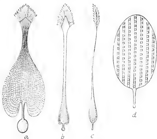
FIG. 53. Scent-scales of diurnal butterflies. a , of Pieris . b , of Argynnis paphia . c , of a Satyrid . d , of Lycaena . All highly magnified.
