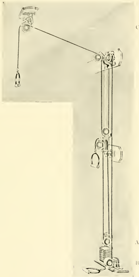
Fig. 28.—Triplex pulley-weight (Narragansett Co.).
