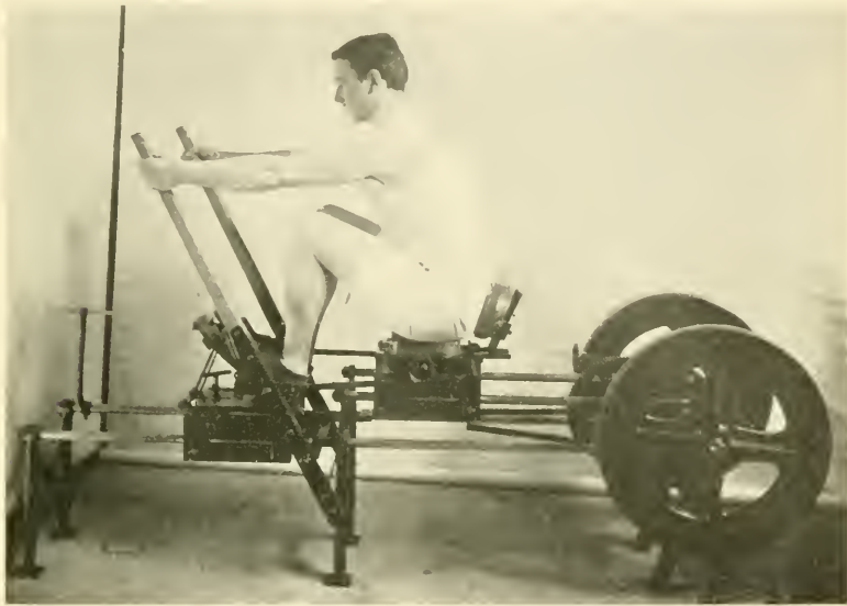
Fig. 36.—The Sargent inomotor with flywheel in place.
