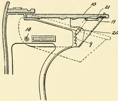
Fig. 118.—Showing mechanism for adjustment of the Garber desk: 10, Adjustable top; 14, pivot of attachment for adjustable portion of top; 18, lever pressed up by fingers to overcome the spring 21 and release the rod 20 from the serrations 9, allowing the desk to be raised or lowered at will.
