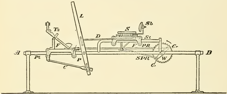
Fig. 35.—The Sargent inomotor.
