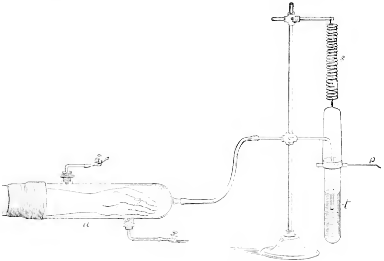
Fig. 6.—A schematic diagram of Mosso's pletysmograph for the arms: a , The glass cylinder for the arm, with rubber sleeve and two tubulatures for filling with warm water; s , the spiral spring swinging the test-tube, t . The spring is so calibrated that the level of the liquid in the test-tube above the arm remains unchanged as the tube is filled and emptied. The movements of the tube are recorded on a drum by the writing point, p . (Howell).
