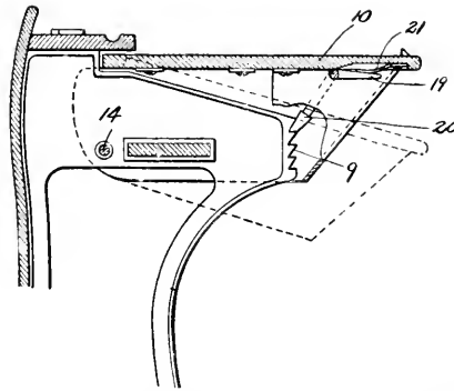
Fig. 118.—Showing mechanism for adjustment of the Garber desk: 10, Adjustable top; 14, pivot of attachment for adjustable portion of top; 16, lever pressed up by fingers to overcome the spring 21 and release the rod 22 from the serrations 20, allowing the desk to be raised or lowered at will.
