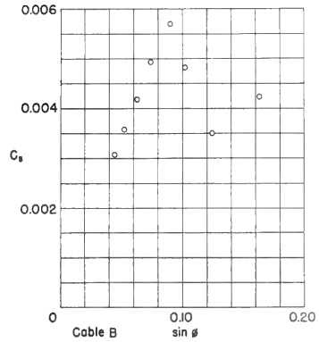
Figure 4b - Cable B, 1/16-inch
