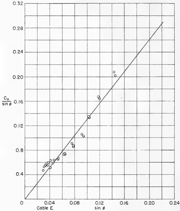
Figure 5 - Variation of \frac{C_n}{\sin^2 \phi} with \sin \phi
