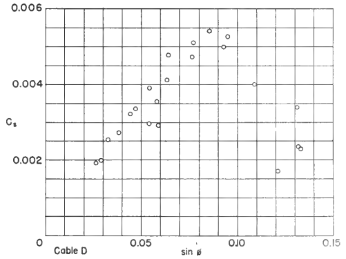
Figure 4d - Cable D, 1/16-inch
