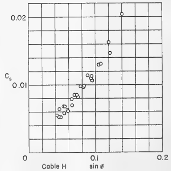
Figure 4h - Cable H, 1/4-inch
