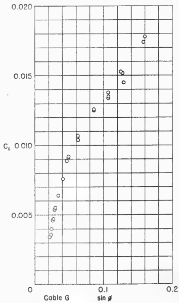
Figure 4g - Cable G, 1/8-inch
