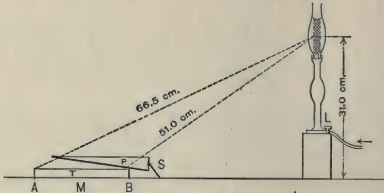
FIG. 59.—Diagram showing the position of apparatus and the direction of the rays in an experiment in phototaxis. T , trough of water containing organisms, A and B its two ends, M its middle. P , a prismatic box containing a solution of India ink. S , screen to cut off extraneous light. L , gas-lamp having a WELSBACH burner. Drawn to scale.
