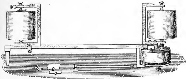
Fig. 26.—Harvard long paper kymograph.
