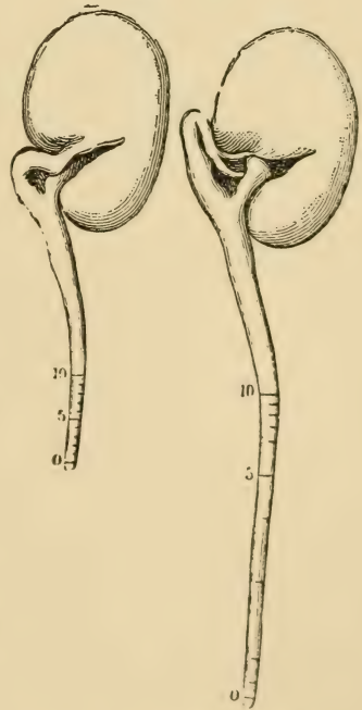
Seedlings of Pea. (Sachs.) Showing zone of maximum growth.
