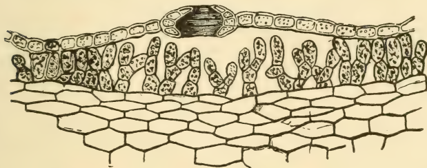
Air-chamber and opening of Marchantia polymorpha : magnified 300 times. (Kerner.)
