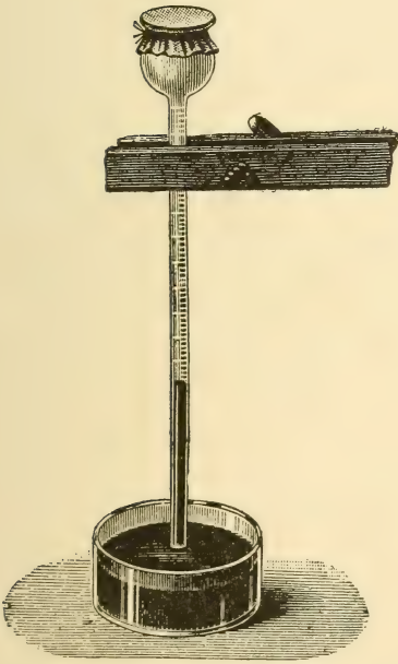
Apparatus to demonstrate lifting power of evaporation. (After Oels.)
