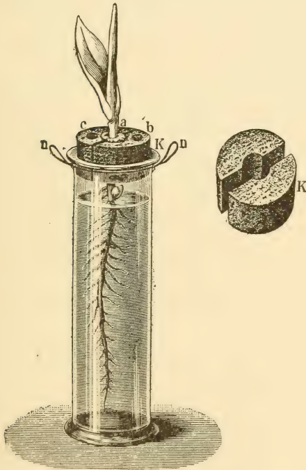
Culture cylinder with seedling of Corn in position. K , cork. (Hansen.)
