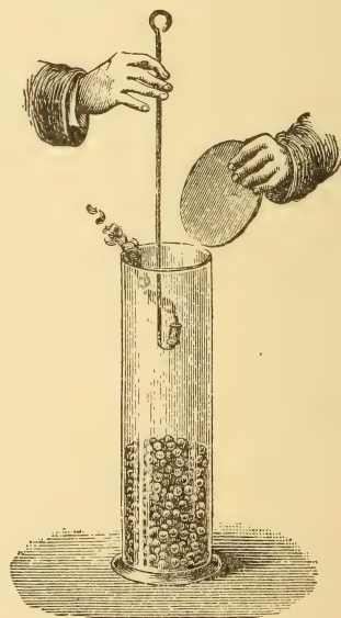
Cylinder containing germinating Peas. (Sachs.)
