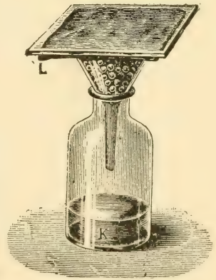
Apparatus to demonstrate progression of zone of root-hairs. (After Oels.) K , potassium hydrate solution; L , moist filter-paper.
