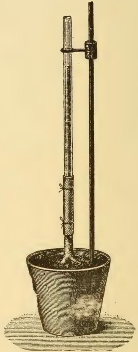
Apparatus for demonstration of root-pressure. (Detmer.)
