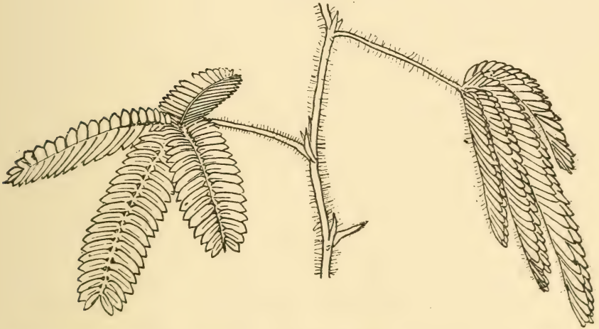
Mimosa pudica . The leaf on the left is in a normal position ; the one on the right has been stimulated. (Detmer.)
