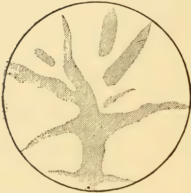
Marble plate corroded by roots. (Detmer.)
