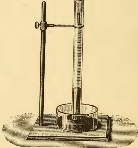
Lifting power of transpiration. (Detmer.)
