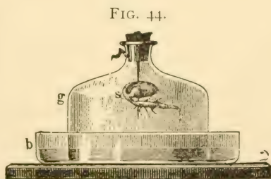
FIG. 44. Progeotropism of seedling. (Determiner.) b , dish partly filled with water; g , bell-glass; s , seedling.
