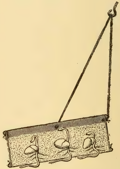
Hydrotropism of roots. (Detmer.)
