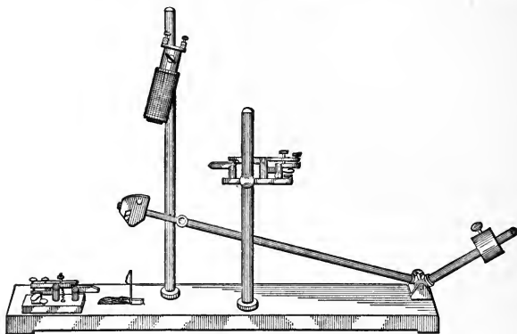
FIG. 52. Simple control hammer.
