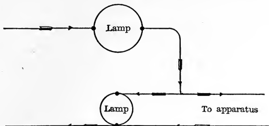
FIG. 36. Schema of lamp battery.
