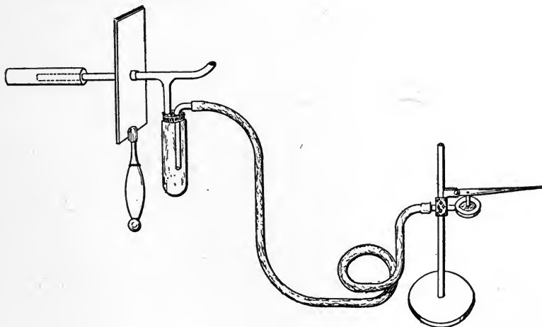
FIG. 67. Zwaardemaker's arrangement for olfactory reactions.
