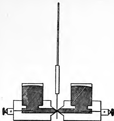
FIG. 57. Krille's interruptor.
