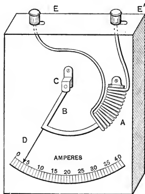
FIG. 38. Ammeter. From S. Bottone, Electricity and Magnetism , 1893, 153.
