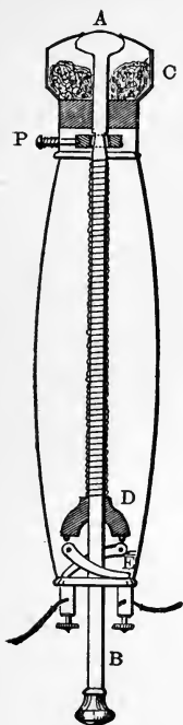
FIG. 66. Buccola's smell stimulator.
