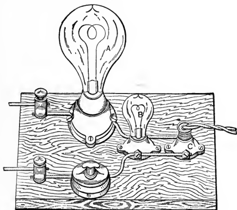
FIG. 37. Lamp battery.
