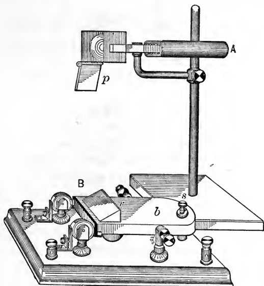
FIG. 53. Sound stimulator.
