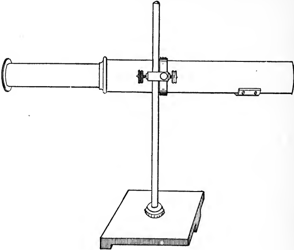
FIG. 82. Reading telescope.
