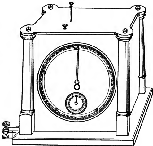
FIG. 43. Münsterberg's chronoscope.
