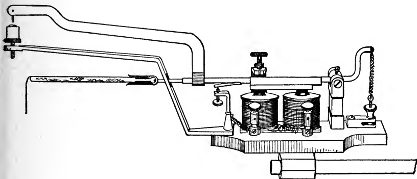
FIG. 50. Kiesow's electroaesthesiometer.
