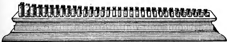
Fig. 5.—Appunn's series of high forks, for the determination of the qualitative TR. The forks are actuated by bowing across the tops of the tines.
