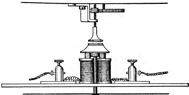
FIG. 42. Mechanism of d'Arsonval chronometer (Philippe).
