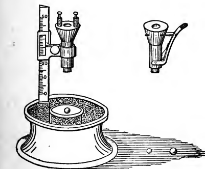
FIG. 8.—Zoth's acoumeter.
