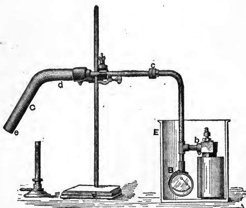
FIG. 217.—CHARGING CALORIMETER WITH OXYGEN.
