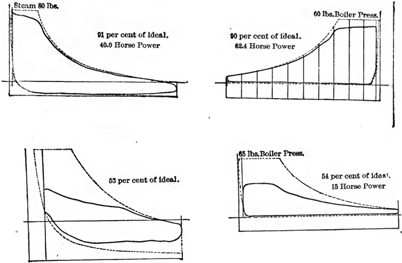
FIG. 265.—LOSS BY CYLINDER-CONDENSATION.
