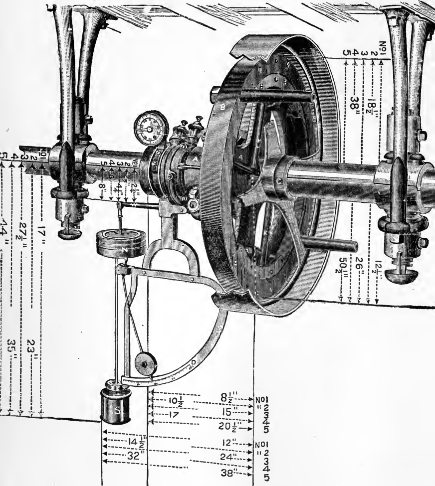
FIG. 135 — EMERSON'S POWER-SCALES.
