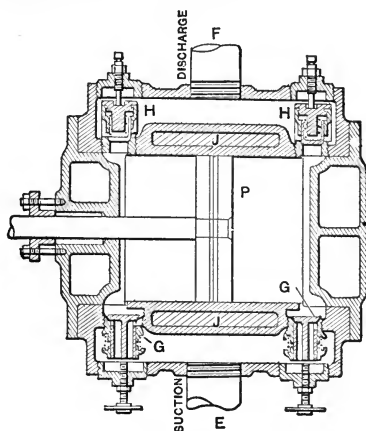
FIG. 323.—AIR-COMPRESSOR CYLINDER.
