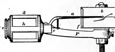
FIG. 291.—THE WILLIAMS INERTIA-INSTRUMENT. PLAN VIEW.
