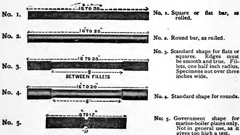
FIG. 85.—FORMS OF SPECIMEN FOR TENSILE STRAINS FORMERLY USED.
