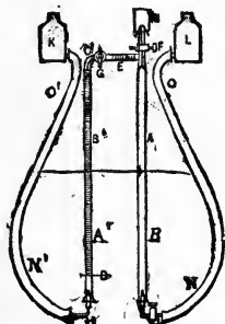
FIG. 216.—ELLIOT'S APPARATUS.
