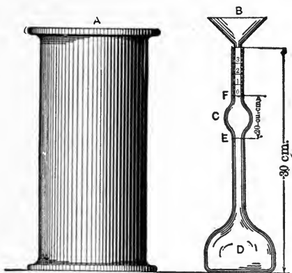
FIG. 99.—LE CHATELIER'S SPECIFIC-GRAVITY APPARATUS.
