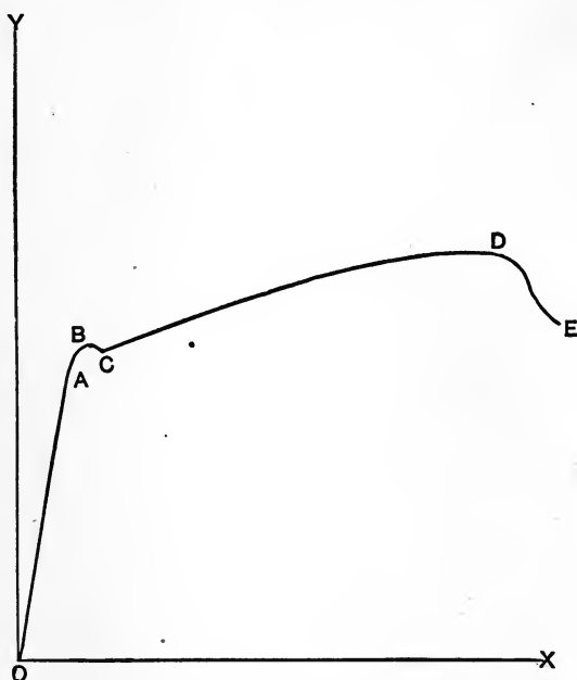
FIG. 27.—THE STRAIN-DIAGRAM.
