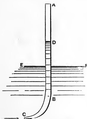
FIG. 144.—PITOT'S TUBE.
