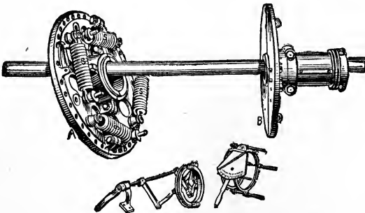
FIG. 137.—PARTS OF THE VAN WINKLE POWER-METER.
