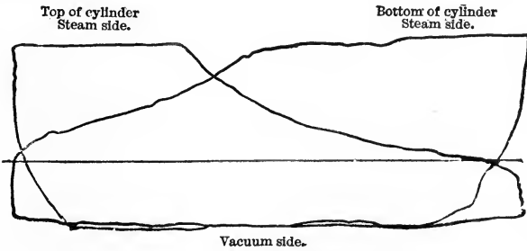
FIG. 266.—UNSYMMETRICAL VALVE-SETTING.
