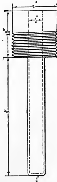
FIG. 190.—THERMOMETER-CUP.
