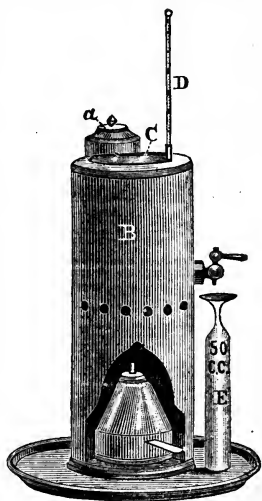
FIG. 103.—TAGLIABUE'S VISCOSIMETER.
