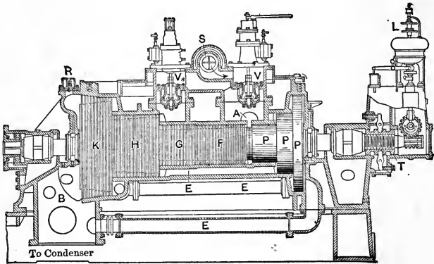
FIG. 307.—PARSONS STEAM-TURBINE.
