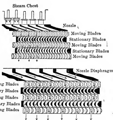
FIG. 308.—NOZZLES AND BUCKETS, CURTIS TURBINE.
