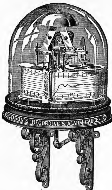
FIG. 174.—EDSON'S SPEED AND PRESSURE RECORDING GAUGE AND ALARM.
