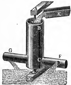
FIG. 157.—THE REACTION-WHEEL.
