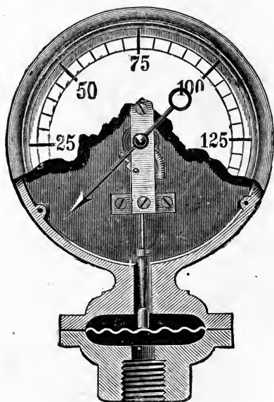
FIG. 172.—DIAPHRAGM-GAUGE.
