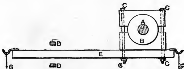
FIG. 118.—PRONY BRAKE.
