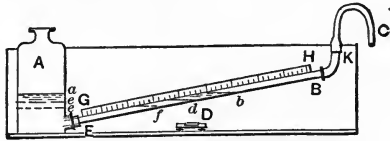
FIG. 165.—DRAUGHT-GAUGE.
