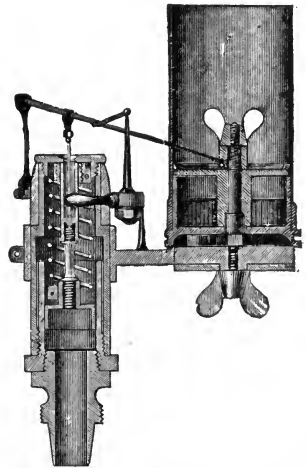
FIG. 230.—SECTION OF THOMPSON INDICATOR.
