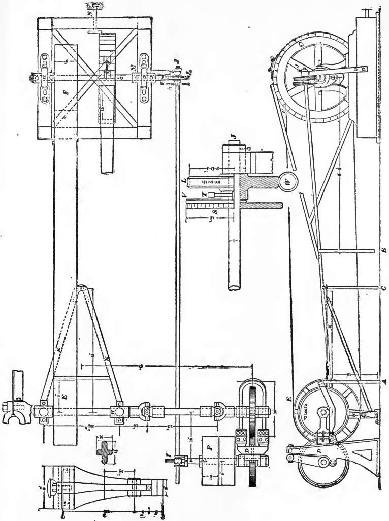
FIG. 139.—BELT-TESTING MACHINE OF SIBLÉV COLLEGE.
