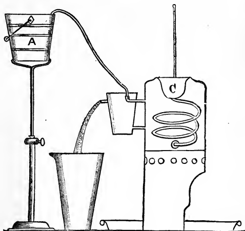
FIG. 104.—TAGLIABUE'S VISCOSIMETER.
