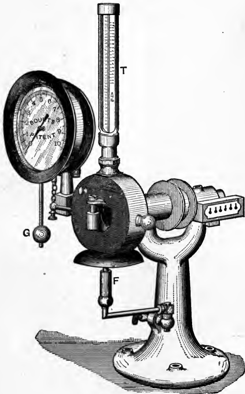
FIG. 115.—BOULTON'S LUBRICANT-TESTER.
