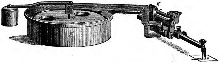
FIG. 12.—SUSPENDED PLANIMETER.
