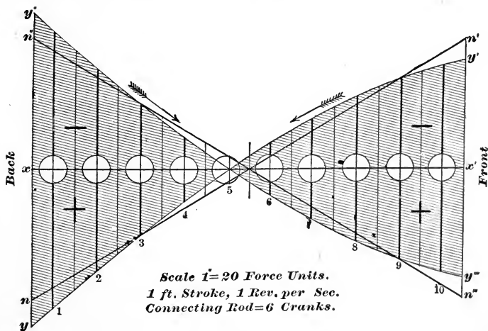
FIG. 297.—INERTIA-DIAGRAMS.
