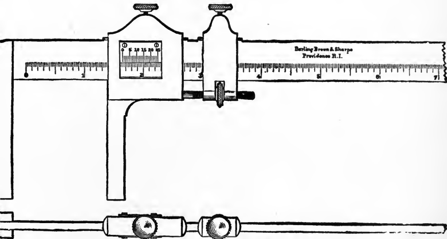
FIG 21.—VERNIER CALIPER.
