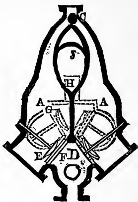
FIG. 303.—THE PULSOMETER.
