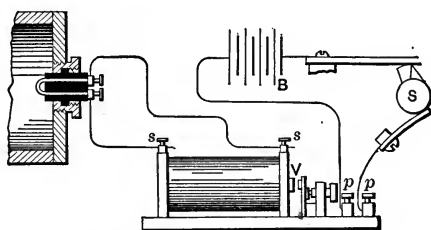
FIG. 316.—JUMP-SPARK IGNITION.
