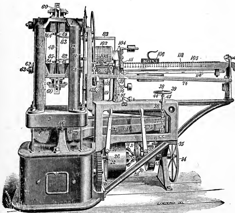
FIG. 56.—THE OLSEN TESTING-MACHINE. FRONT VIEW.
