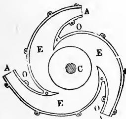
FIG. 158.—SCOTTISH TURBINE.
