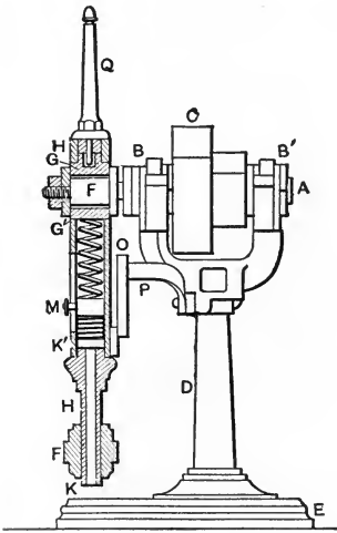
FIG. 109.—SECTION OF THURSTON'S OIL-TESTING MACHINE.
