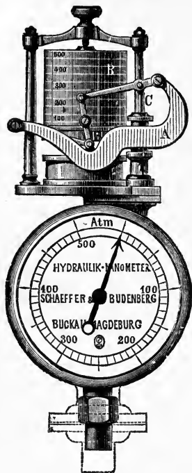
FIG. 175.—RECORDING PRESSURE-GAUGE.
