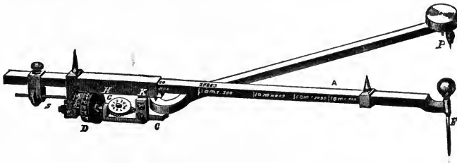
FIG. 4.—AMSLER'S POLAR PLANIMETER.
