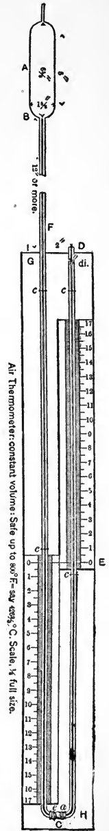
FIG. 181.—THE HEADLEY AIR-THERMOMETER.
