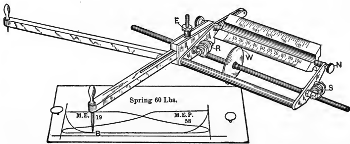
FIG. 14a.—THE WILLIS PLANIMETER.
