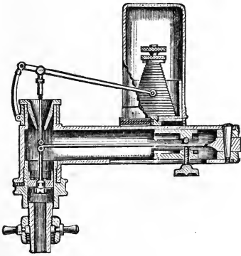
FIG. 235.—THE BACHELDER INDICATOR.
