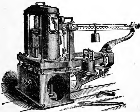
FIG. 54.—HYDRAULIC TESTING-MACHINE.
