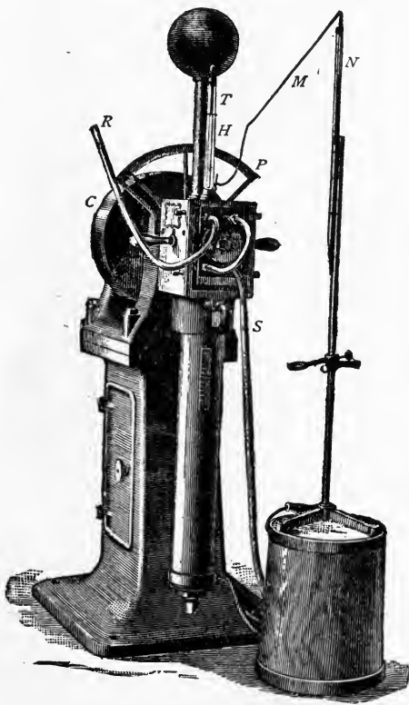
FIG. 111.—THURSTON'S RAILROAD-LUBRICANT TESTING-MACHINE.
