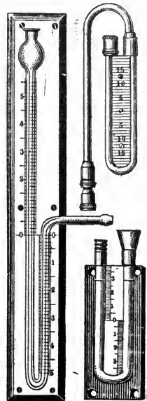
FIG. 160.—U-SHAPED MANOMETER-TUBES.
