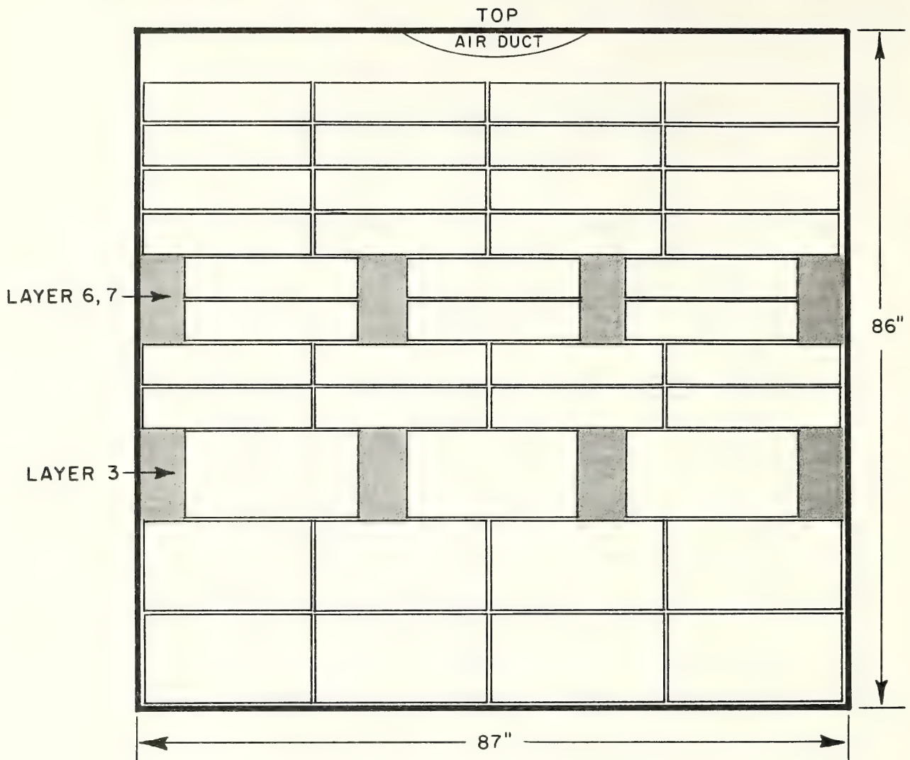
Figure 3.--Rear view of parallel air channel loading pattern used for boxes 30 x 21 x 11 and 30 x 21 x 6 inches (76.2 x 53.3 x 27.9 and 76.2 x 53.3 x 15.2 cm) in layers 3 and 6, 7. Air channels are shaded.
