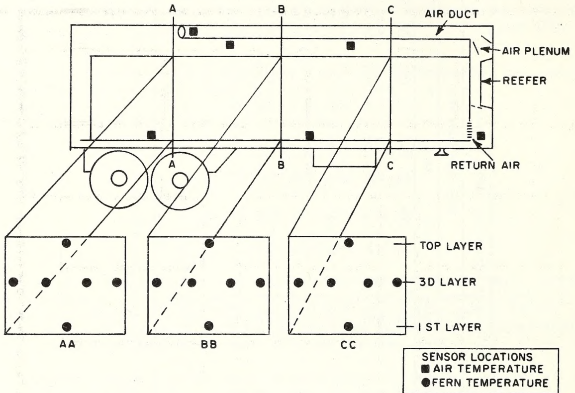
Figure 1.--Location of 6 cargo area air and 18 product temperature sensors in a typical test van container, showing end view through load.
