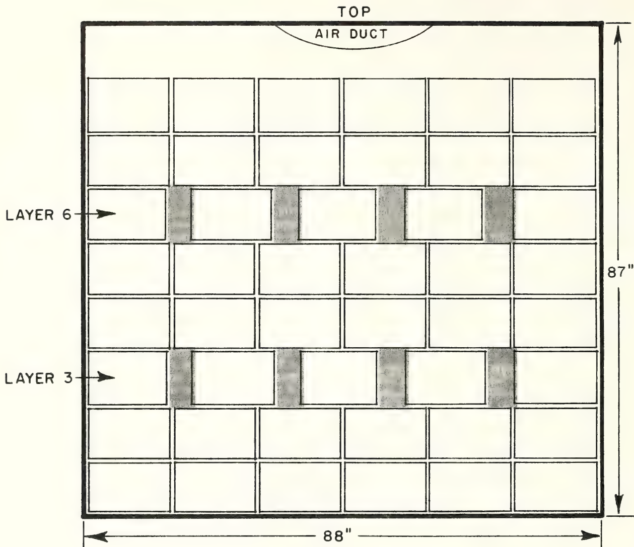
Figure 5.--Rear view of parallel air channel loading pattern used for boxes 30 x 14 x 9 inches (76.2 x 35.6 x 22.9 cm). Air channels in layers 3 and 6 are shaded.
