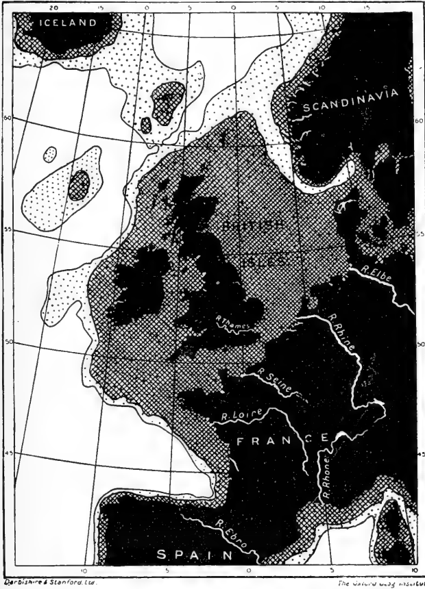
FIG. 26.—Map to show the effect of elevation of the earth's surface on the distribution of land and water in Western Europe. The doubly-cross-shaded area shows what would become dry land if the sea-bottom were raised 600 feet. The Channel, the German Ocean, the Baltic and the Irish Sea, cease to exist. The smaller dotted area would become dry land if the sea-bottom rose another 2,400 feet. Men could then walk from Scotland to Iceland by way of the Shetlands and Faroe Islands. Most noticeable is the great change which would be brought about by the comparatively small rise of 600 feet, and the much greater elevation required to change any further the contour of the land.
