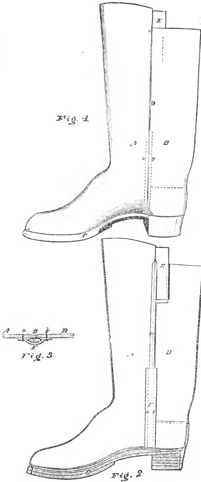
Fig. 1 represents the outside of the Boot. Fig. 2 " " " inside " " Fig. 3 " " a section of the Seam.
