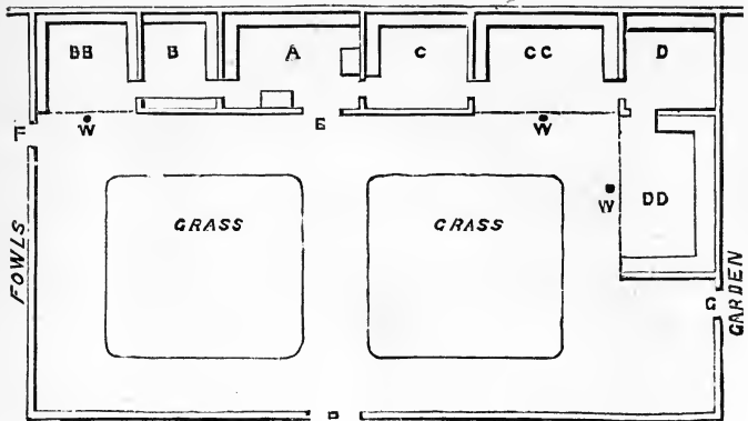
FIG. 6.—PLAN OF SMALL PIGEONRY.
