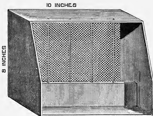
FIG. 10.—SALT EARTH BOX FOR PIGEONS.
