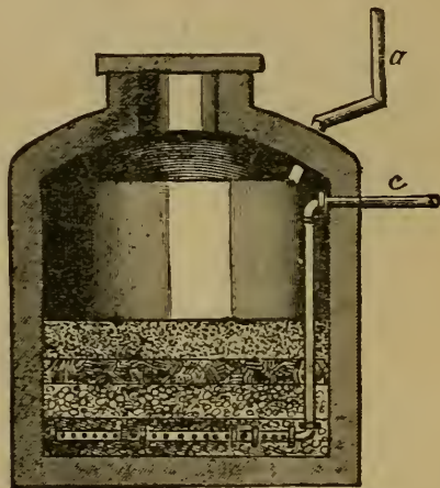
Fig. 146.—A HOUSE FILTERING CISTERN.
