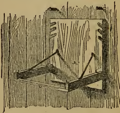
Fig. 65.—A BETTER BAG HOLDER.
