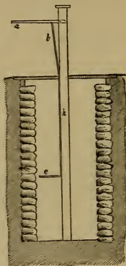
Fig. 130.—AGITATOR FOR WELL.
