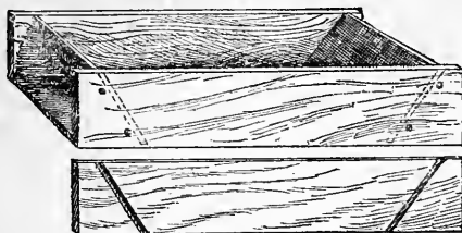
Fig. 27.—A PLANK WATER TROUGH.
