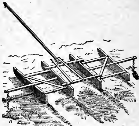
Fig. 59.—A HORSE LAND-MARKER.
