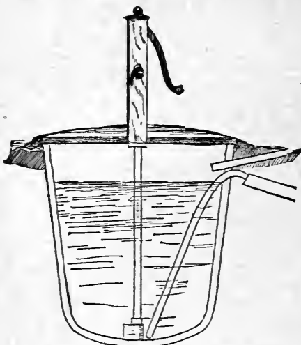
Fig. 137.—FROST-PROOF CISTERNS.
