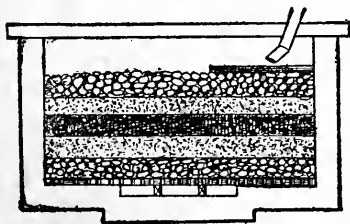
Fig. 145.—FILTER FOR A BARN CISTERN.
