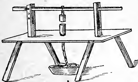
Fig. 233.—A SAUSAGE FILLER.
