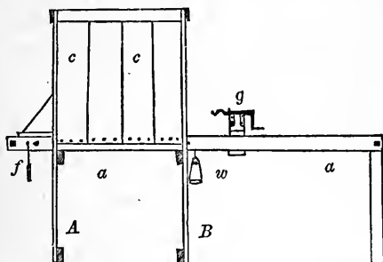
Fig. 167.—THE COMPLETE MACHINE (STRAW-TWISTER).
