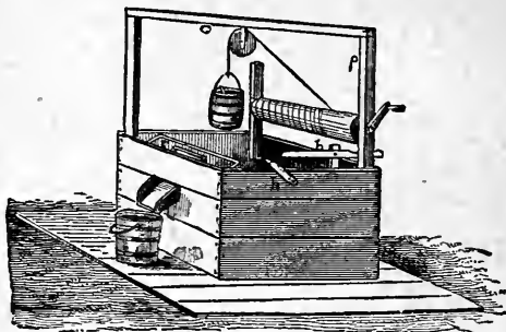
Fig. 122.—IMPROVED WINDLASS.
