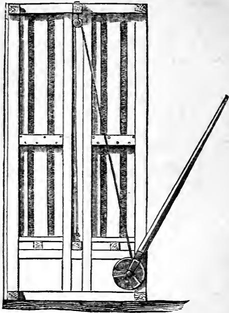
Fig. 160.—END VIEW OF HAY PRESS.
