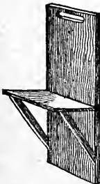
Fig. 111.—MILKING STOOL.
