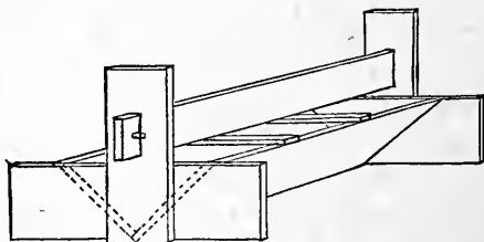
Fig. 19.—DOUBLE FEEDING TROUGH FOR PIGS.
