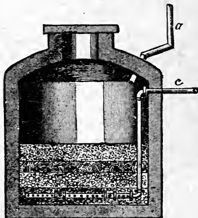
Fig. 146.—A HOUSE FILTERING CISTERN.
