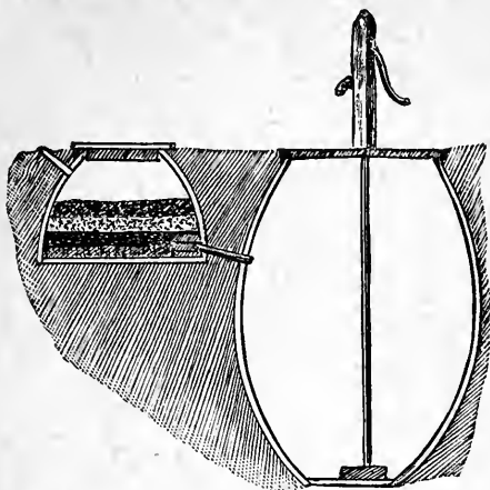
Fig. 144.—COMPLETE CISTERN AND FILTER.
