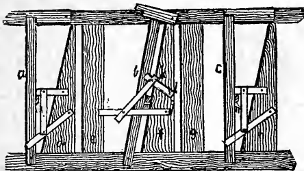
Fig. 8.—SELF-CLOSING CATTLE STANCHION.
