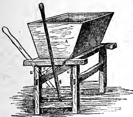
Fig. 86.—HOME-MADE ROOT-CUTTER. Fig. 87.—ROOT-CUTTER SLIDE.
