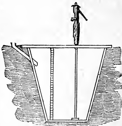
Fig. 143.—A COMPLETE CISTERN.
