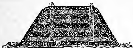
Fig. 192.—PIT FOR BURNING MARL.
