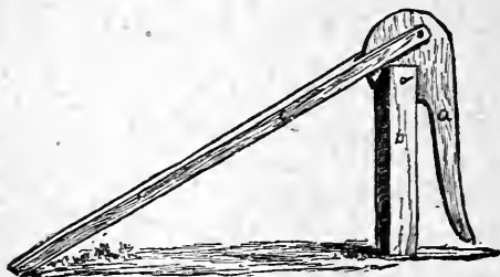
Fig. 40.—HOME-MADE WAGON-JACK.
