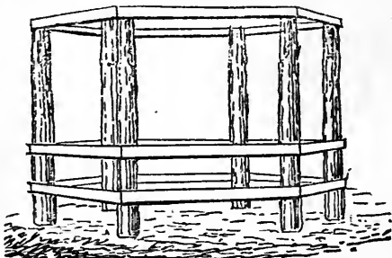
Fig. 158.—FRAME FOR STRAW OR HAY STACK.
