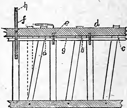
Fig. 9.—DEVICE FOR CLOSING CATTLE STANCHIONS.
