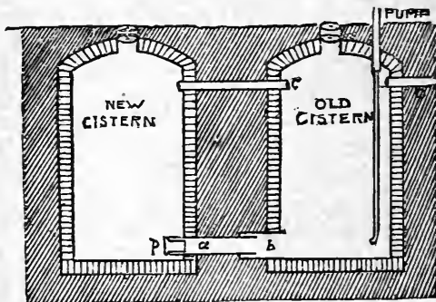
Fig. 142.—CONNECTING TWO CISTERNS.
