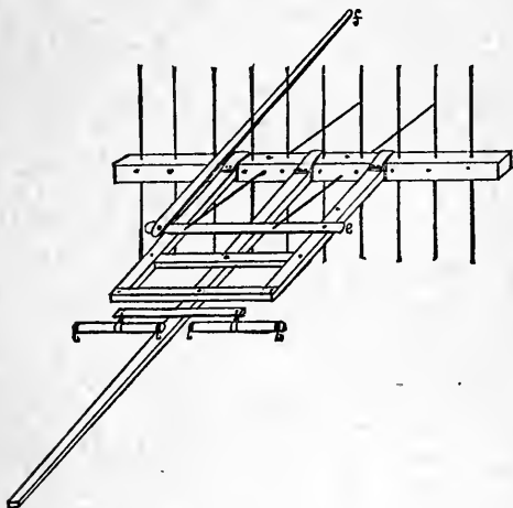
Fig. 150.—RAKE FOR TWO HORSES.
