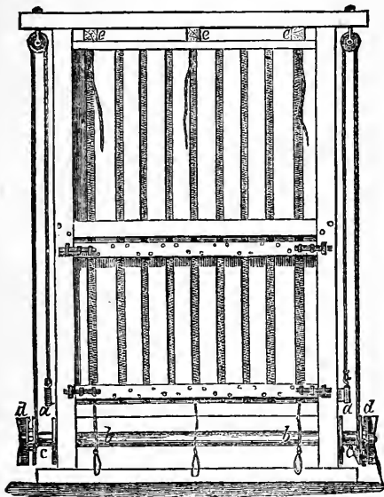
Fig. 159.—FRAME OF HAY PRESS.
