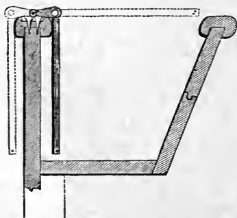
Fig. 2.—IMPROVED HORSE MANGER.
