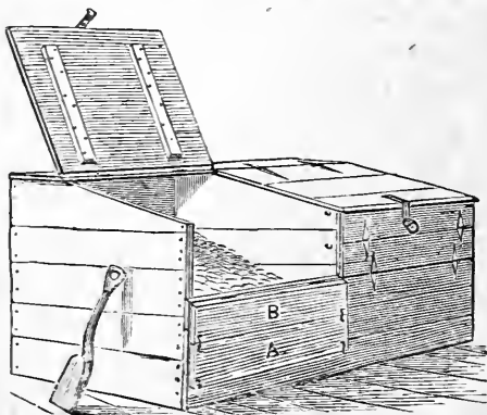
Fig. 24.—CONVENIENT GRAIN BIN.
