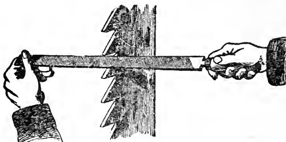
Fig. 100.—PROPER METHOD OF FILING.
