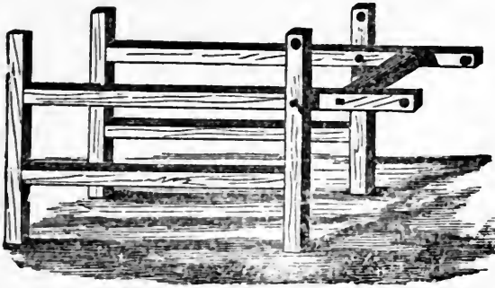
Fig. 58.—STALL FOR BULL.
