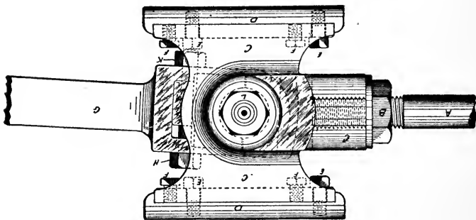
CROSS-HEAD.
