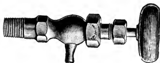
TRY COCK.
