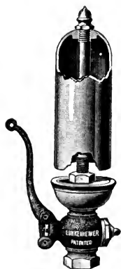
PLAIN WHISTLE.
