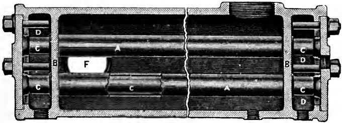
SECTIONAL VIEW OF CASE HEATER.
