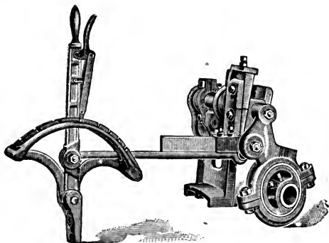
HUBER SINGLE ECCENTRIC REVERSE.
