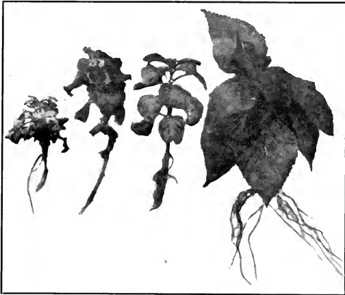
FIG. 32.—Green-wood cuttings.
