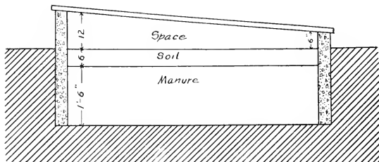
FIG. 11.—A cross-section of a concrete hotbed.
