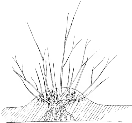
FIG. 26.—Mound layering.
