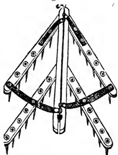
Geddes Harrow.
