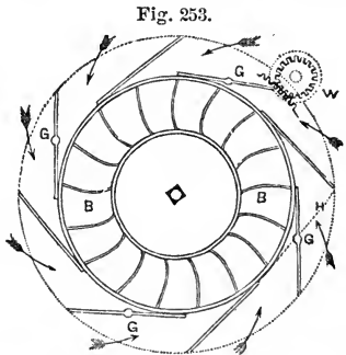
Section of Van de Water Wheel. buckets separate.
