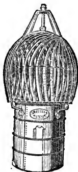
Griffith's Ventilator.
