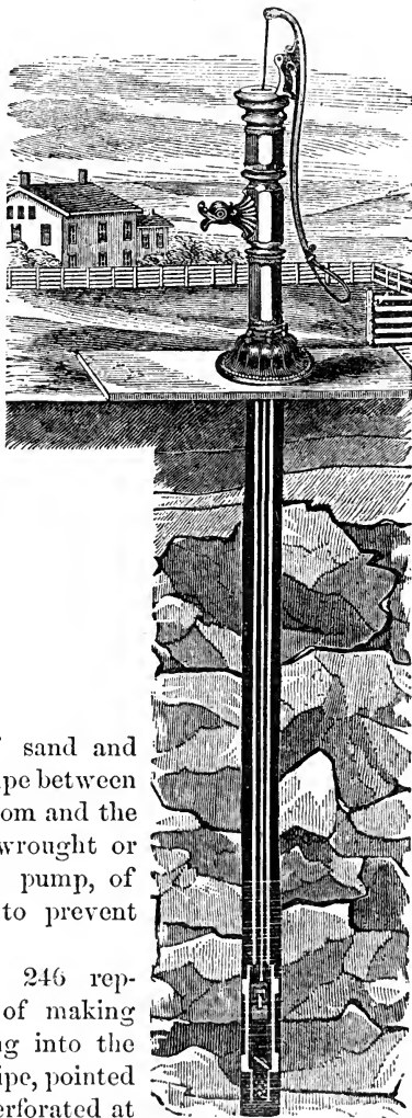
Deep-well Pump.
