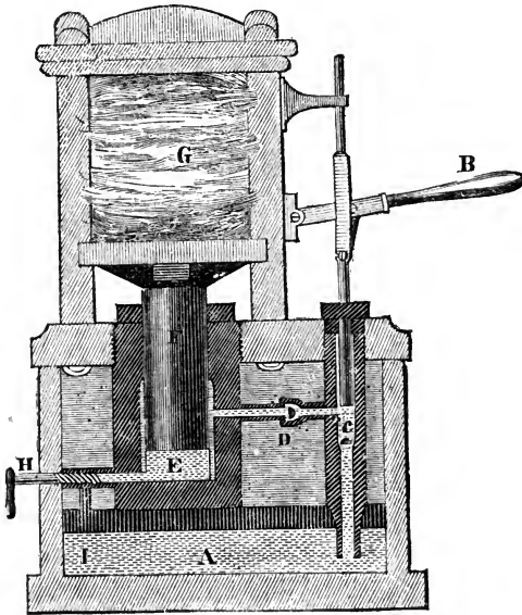
Hydrostatic Press.
