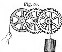
Combined cog-wheels.
