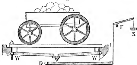
Weighing Machine.
