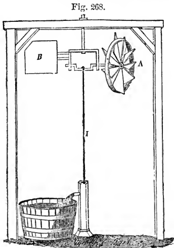
Wind-mill for pumping water on farms : A, wind-mill; B, vane; I, pump-rod.
