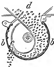
Cross-section of Seed-holder.
