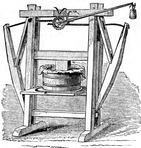
Kendall's Cheese-press.
