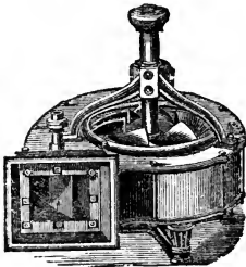
View of Reynolds' Turbine Wheel.
