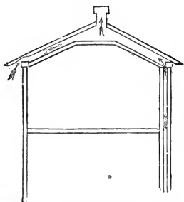
Mode of Ventilating half-story Bed-rooms.
