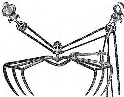
Raymond's Fork.
