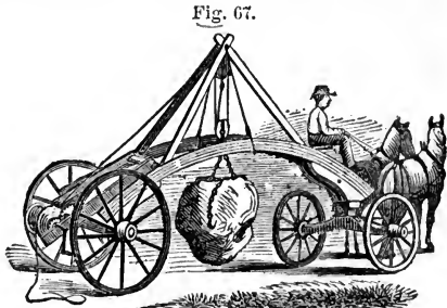
Fig. 67. Packer's Stone Lifter.
