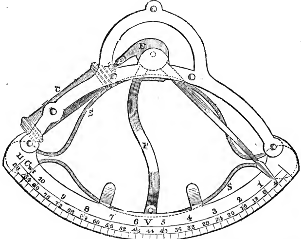
Elliptic Dynamometer, in compact form: S S, spring; F, cross-lever for moving index
