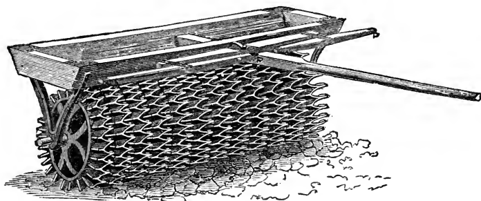
American Clod-crusher.
