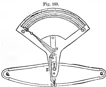
Elliptic Dynamometer.
