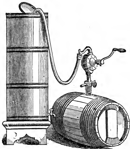
Rotary Pump, for Barrels, etc.
