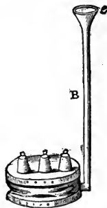
Hydrostatic Bellows.
