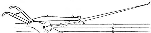
Line of draught for the plow.
