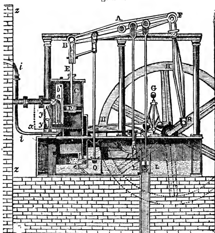
Low-pressure Steam-engine.
