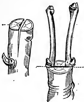
FIG. 124.—CLEFT-GRAFTING.
