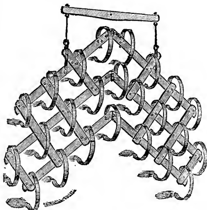
FIG. 67.—SPRING TOOTH HARROW.
