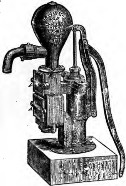
FIG. 88.—EXCELSIOR SUCTION AND FORCE-PUMP.
