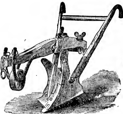
FIG. 59.—ADAMANT PLOW.
