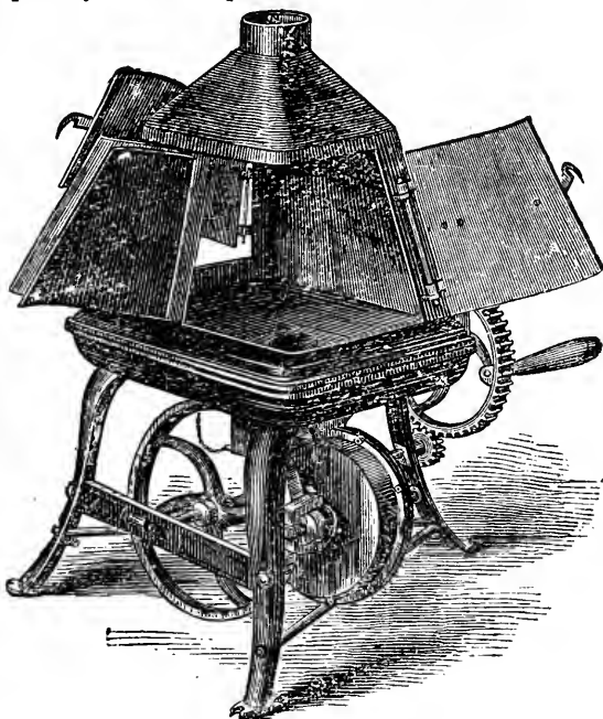
FIG. 81.—EMPIRE PORTABLE FORGE.
