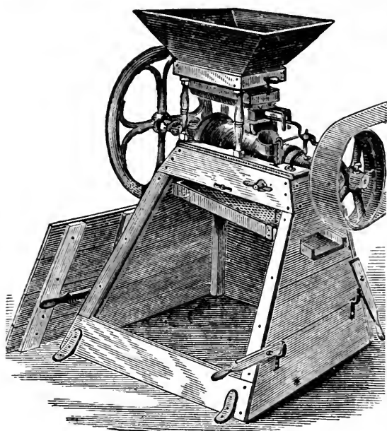
FIG. 76.—BOYER'S PORTABLE FARM GRIST-MILL.
