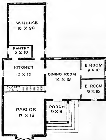
FIG. 3.—PLAN OF GROUND-FLOOR.
