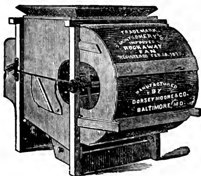
FIG. 73.—ROCKAWAY FAN.
