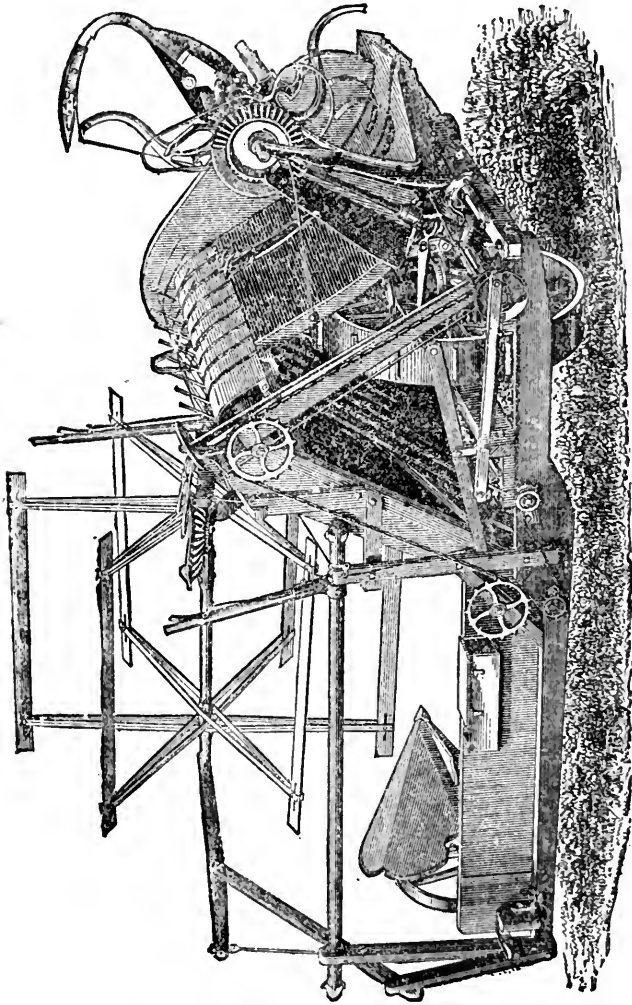
FIG. 19.—WALTER A. WOOD'S SELF-BINDING HARVESTER.
