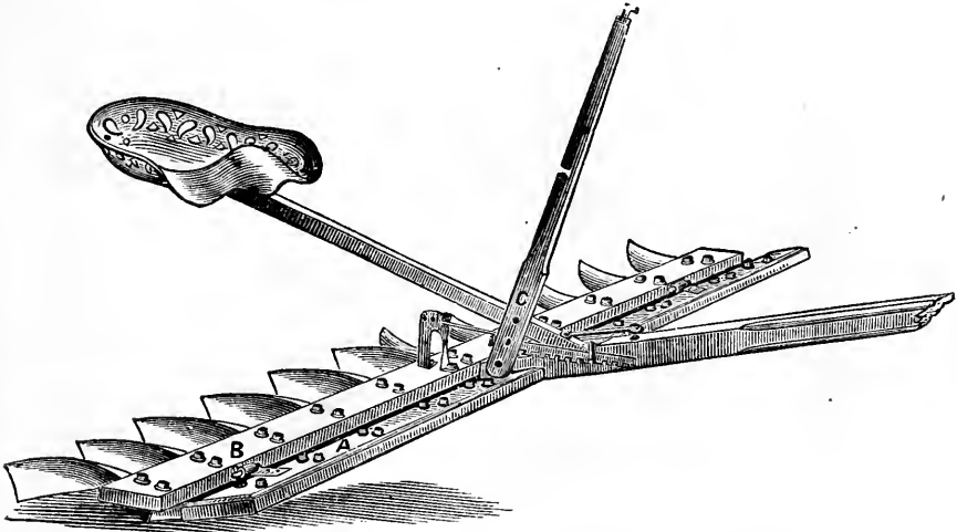
FIG. 68.—ACME CLOD-CRUSHER, LEVELER AND PULVERIZER.
