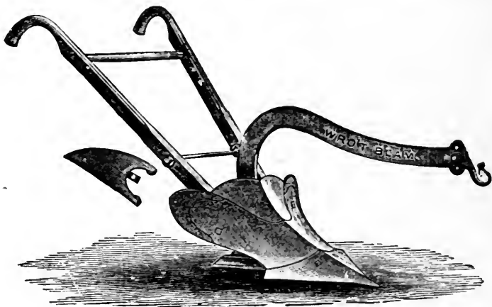
FIG. 34.—DOUBLE-MOULD BOARD-PLOW.
