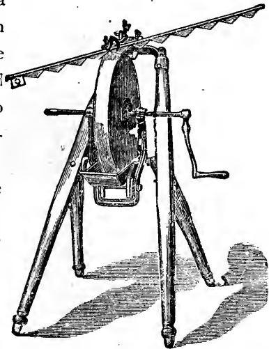
FIG. 78.—SICKLE GRINDER.
