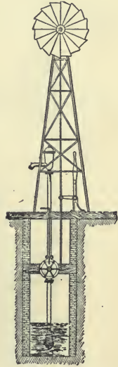
FIG. 82—BERLIN OSCILLATING PUMP.
