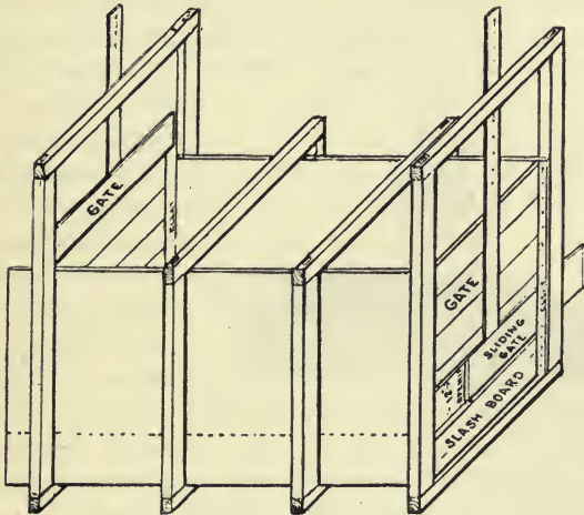
FIG. 47—LATERAL BULKHEAD.
