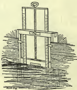
FIG. 45—THE STOKES MEASURING GATE.
