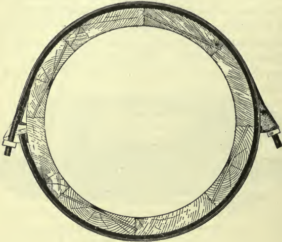
FIG. 27—CROSS-SECTION OF STAVE PIPE.
