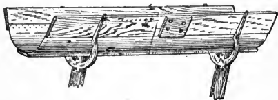
FIG. 35—SIDE VIEW OF SMALL IRON FLUME.
