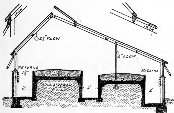
FIG. 109—GREENHOUSE IRRIGATION.
