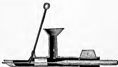
FIG. 25—ASBESTINE PIPE MACHINE.
