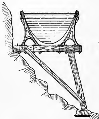
FIG. 38—FLUME ON A ROCKY LEDGE.
