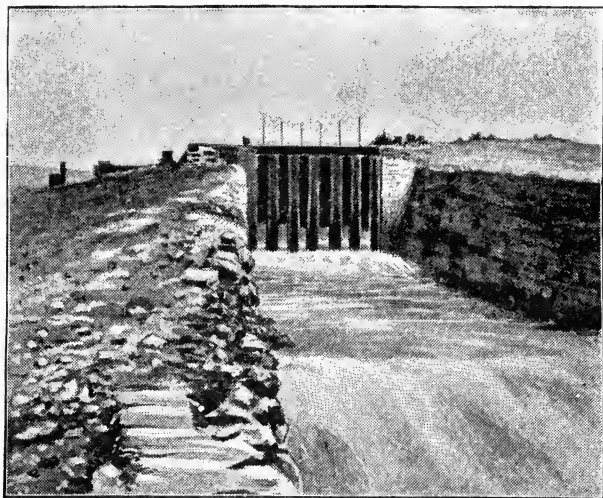
FIG. 12—HEADGATE OF A CANAL
