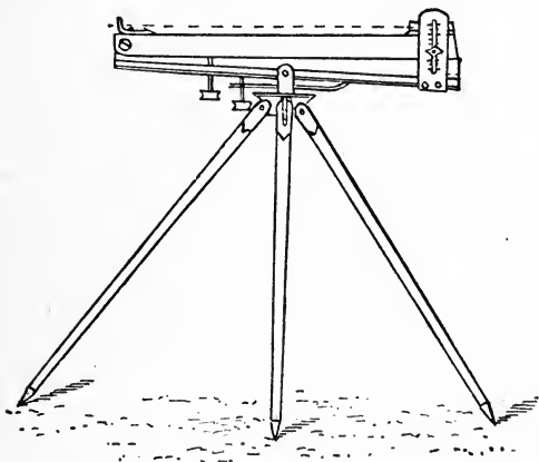
FIG. 7—THE JACKSON LEVEL.
