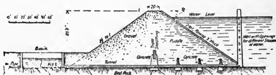
FIG. 21—CROSS-SECTION OF HYDRAULIC RESERVOIR.
