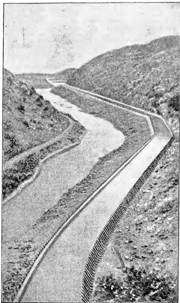
FIG. 33—BENCH FLUME FOR A LARGE CANAL.
