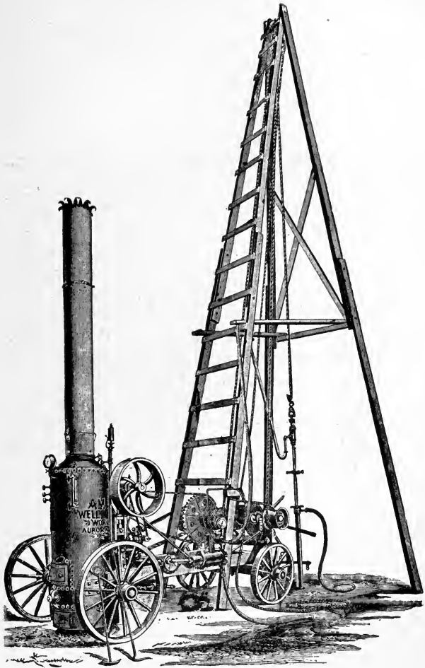
FIG. 94—ARTESIAN DRILLING OUTFIT.
