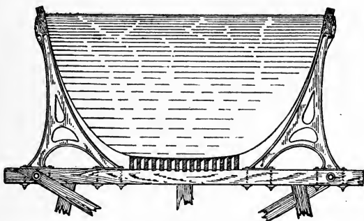
FIG. 37—CROSS-SECTION OF LARGE IRON FLUME.
