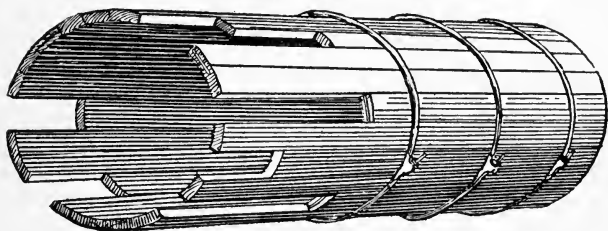
FIG. 26—SIDE VIEW OF STAVE PIPE.
