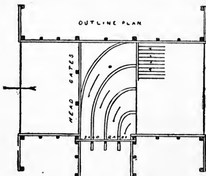
FIG. 13—TOP SECTIONAL VIEW OF LAND'S SAND GATE.
