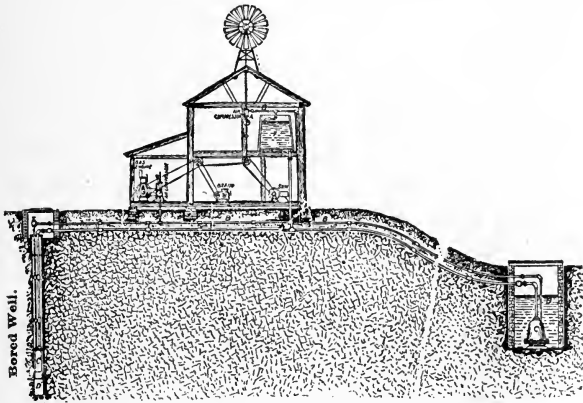
FIG. 91—THE PNEUMATIC SYSTEM.
