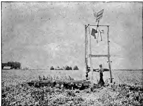
FIG. 78—BATTLE-AX WINDMILL.
