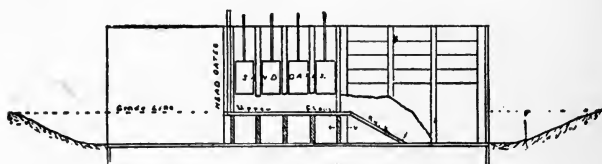
FIG. 14—SIDE VIEW OF SAND GATE.
