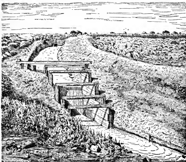
FIG 9—DROP AND REDUCTION BOX.
