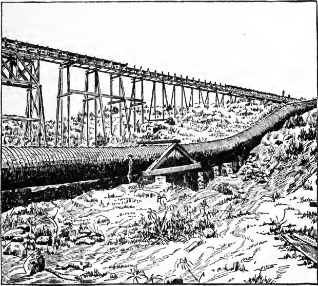
FIG. 28—STAVE PIPE-LINE IN POSITION.
