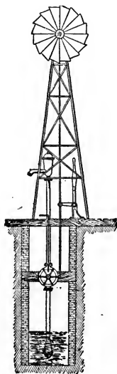
FIG. 82—BERLIN OSCILLATING PUMP.
