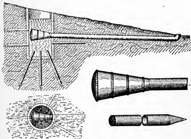
FIG. 6—THE NEWSOM SYSTEM OF WATER-SUPPLY.
