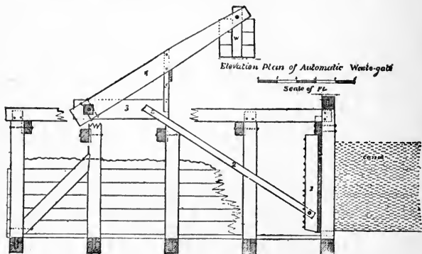
FIG. 16—AUTOMATIC WASTE GATE.
