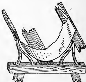
FIG. 36—END VIEW OF SMALL IRON FLUME.
