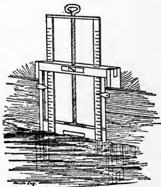
FIG. 45—THE STOKES MEASURING GATE.
