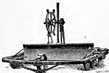
FIG. 48—IMPROVED STEEL LAND GRADER.
