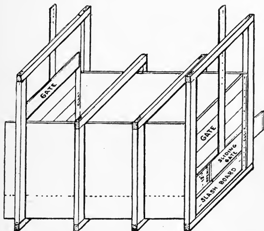
FIG. 47—LATERAL BULKHEAD.
