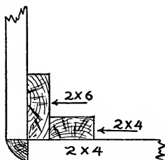
Figure 215.—Corner Post Detail of Horse Feeding Rack. A 2x6 is spiked into the edge of a 2x4, making a corner post 6" across. The side boarding is cut even with the corner of the post and the open corner is filled with a two-inch quarter-round as shown.
