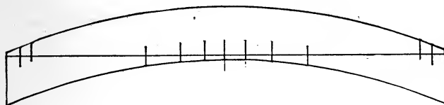
Figure 184.—Diagram showing how to cut a plank on a band-saw to form a curved rafter. The two pieces of the plank are spiked together as shown in the lower drawing. This makes a curved rafter without waste of material.
