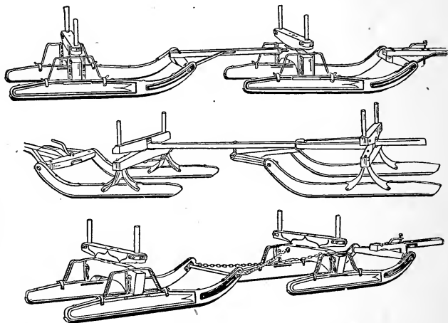
Figure 167.—Bobsleighs, Showing Three Kinds of Coupling. The upper sleighs are coupled on the old-fashioned short reach plan except that the reach is not mortised into the roller. It is gained in a quarter of an inch and fastened by an iron strap with a plate and nuts on the under side. The bobs in the center show the bolster reach, principally used for road work. The bottom pair are coupled by cross chains for short turning around trees and stumps in the woods.
