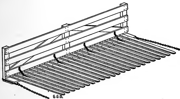
Figure 145.—Buck Rake. When hay is stacked in the field a four-horse buck rake is the quickest way to bring the hay to the stack. The buck rake shown is 16 feet wide and the 2x4 teeth are 11 feet long. Two horses are hitched to each end and two drivers stand on the ends of the buck rake to operate it. The load is pushed under the horse fork, the horses are swung outward and the buck rake is dragged backward.
