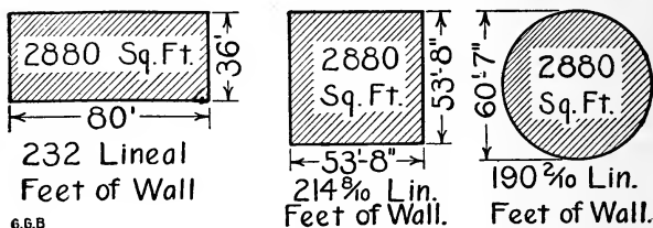
Figure 172.—Economy of Round Barn. The diagrams show that the popular 36'x80' cow stable and the commonest size of round barn have about the same capacity. Each barn will stable forty cows, but the round barn has room for a silo in the center. Both barns have feed overhead in the shape of hay and straw, but the round feed room saves steps.
