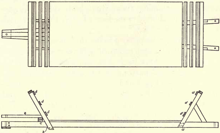
FIG. 101. — WORKING DRAWINGS OF CORN RACK.
