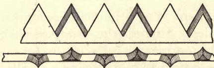
FIG. 149.—TEETH OF A CROSSCUT SAW.
