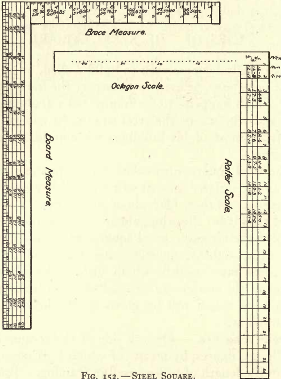
FIG. 152. — STEEL SQUARE.
