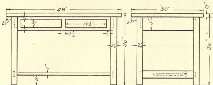
FIG. 249.—LIBRARY TABLE.
