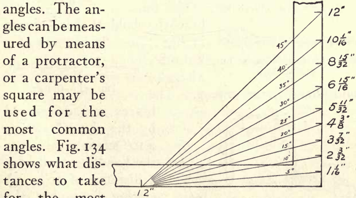
FIG. 134.—DISTANCES TO BE USED IN SETTING BEVEL AT THE MOST COMMON ANGLES.
