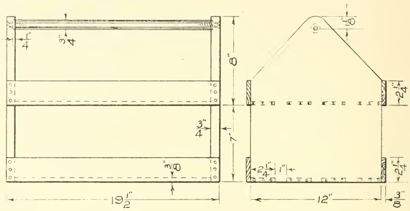
Double Deck Berry Stand (for twelve boxes)
