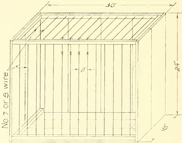
Poultry Show Crate
