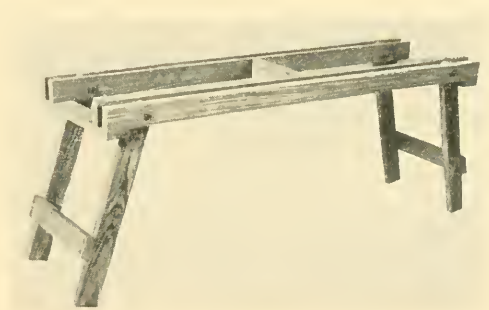
Fig. 8A. Folding Bench.
