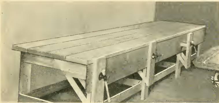
Fig. 5. Rural School Work Bench with Six Vises.
