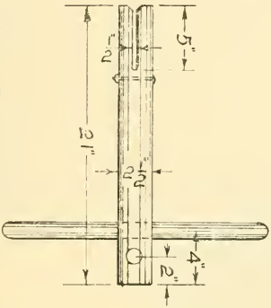
Wire Tightener (Hickory or other tough wood)
