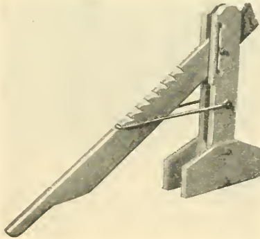
Fig. 10. Wagon Jack.
