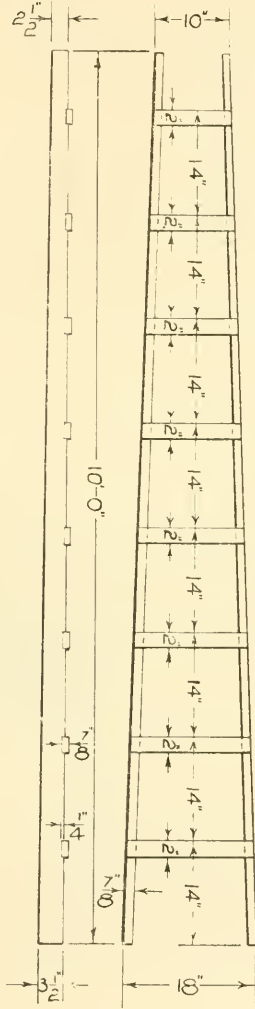
Handy Ladder (Oak, ash, maple or other hardwood)
