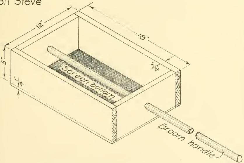
Soil Sieve
