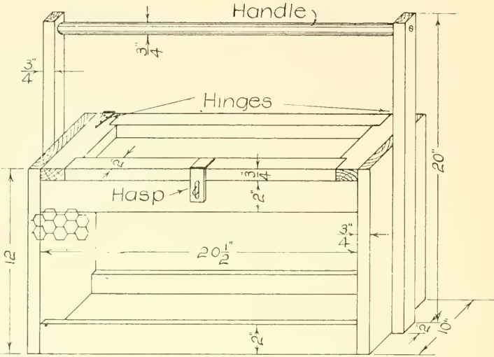
Poultry Carrying Crate
