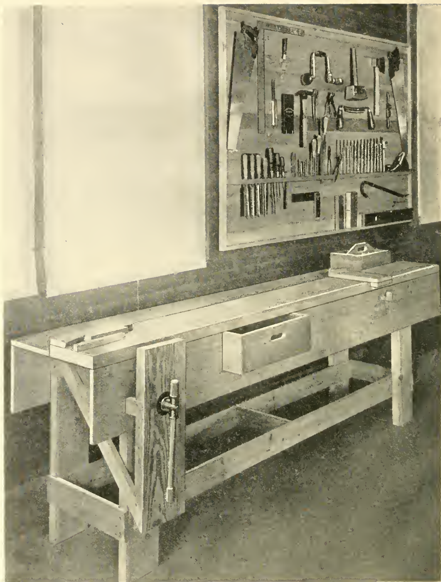
Farm Shop Work Bench and Farm Woodworking Tools.
