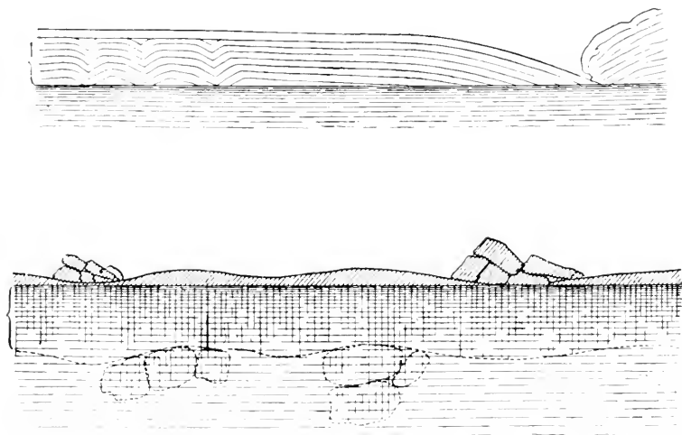
DIAGRAMS OF ICE WITH LAYERS
