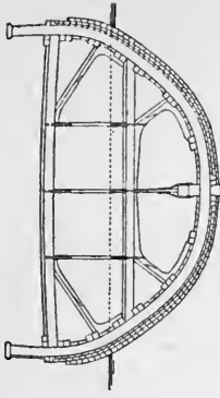
Fig. 3. Transverse section amidships.
