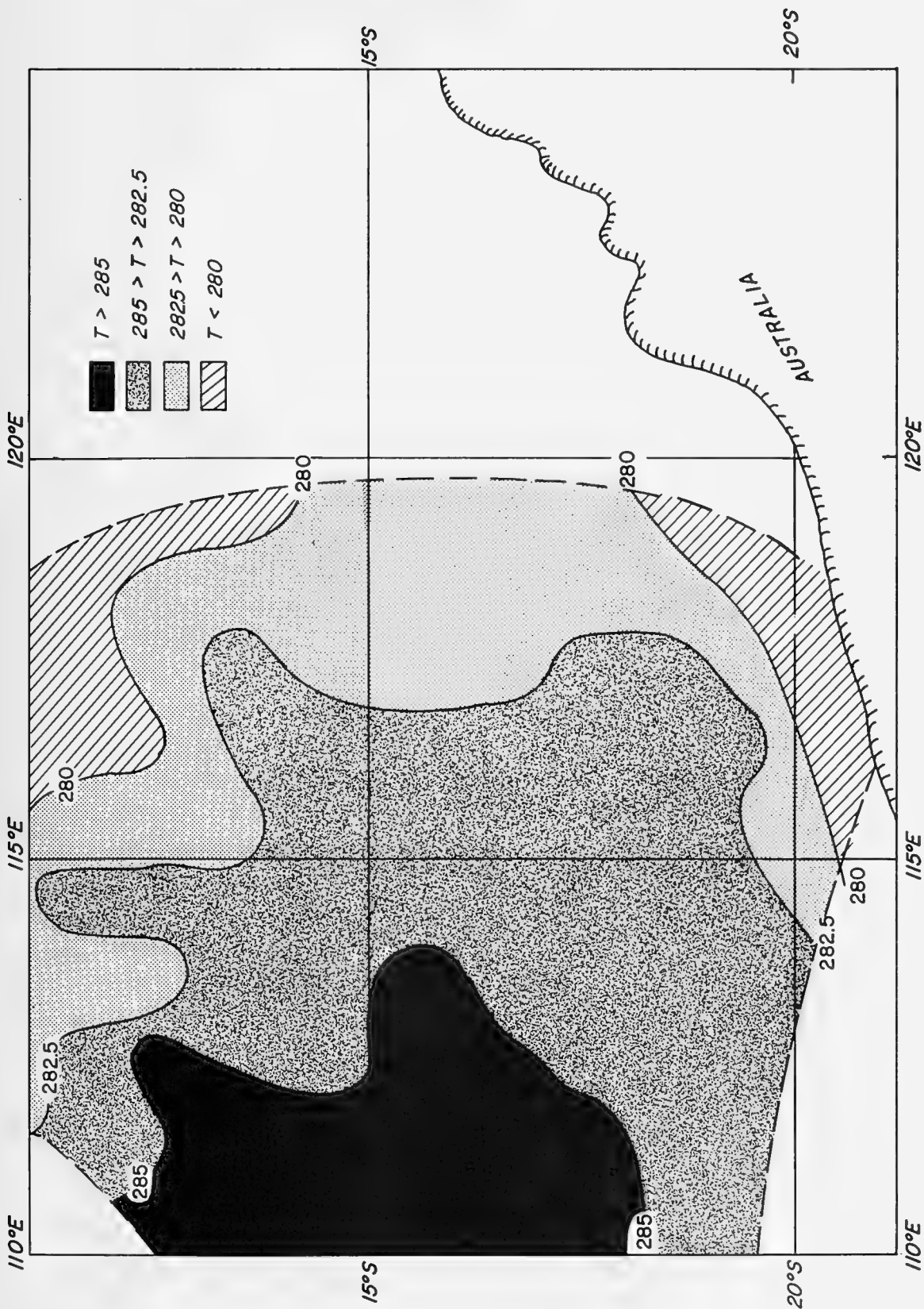
Fig. 5-9 Indian Ocean, Night-time Pass 744 (8 August, 1963)
