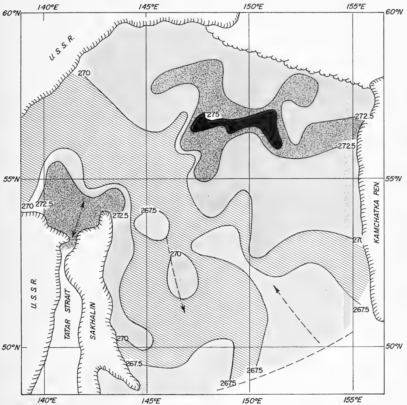
Fig. 5-4 Sea of Okhotsk, Pass 51 (22 June, 1963)
