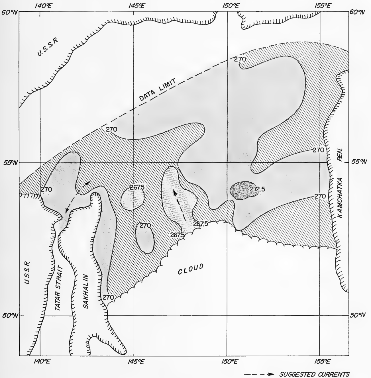
Fig. 5-5 Sea of Okhotsk, Pass 65 (23 June, 1963)
