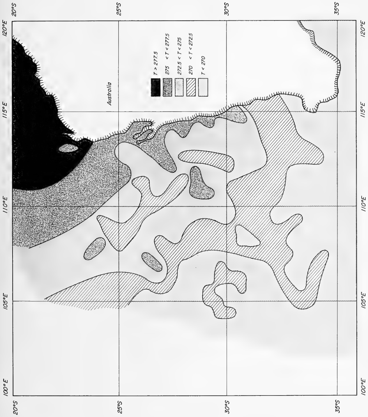
Fig. 6-1 Six Pass Averaged SST Patterns (29 July - 8 August, 1963)
