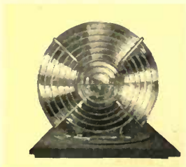
Fourth Order Two Panel Bivalve Lens
