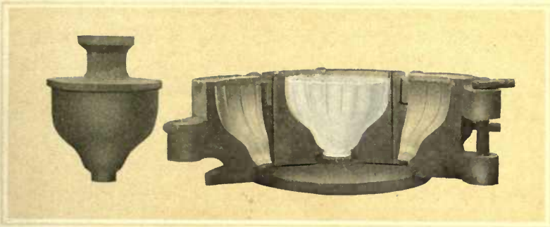
Press Mold Showing Plunger
