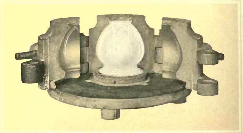
Iron Blow Mold
