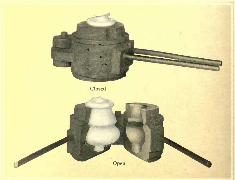
Paste Blow Mold
