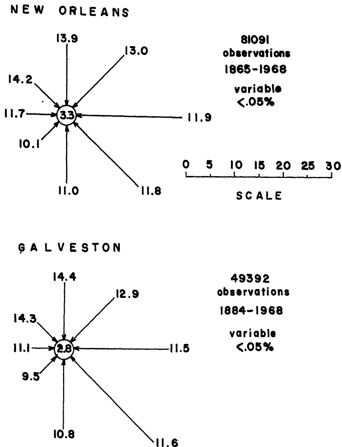
Figure 12. Annual wind patterns from two localities along the northern coast of the Gulf of Mexico. (Data source: U.S. Naval Weather Service Command, 1970 a, b) Numbers at the ends of the arrows indicate average velocity in knots; number at the center is the percentage occurrence of calms. Length of arrows indicate percentage occurrence of winds from that direction.
