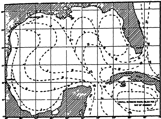
Figure 17 Surface currents in the Gulf of Mexico in June (From Laipper, 1954).
