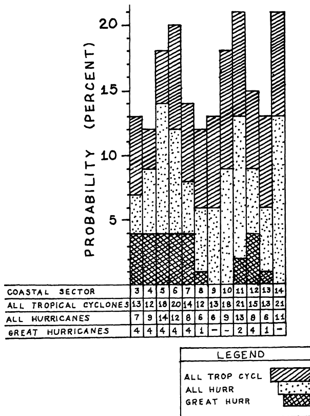
Figure 14. Cyclone probabilities for coastal sectors along the Gulf Coast (From Simpson and Lawrence, 1971). See Figure 13 for location of indicated coastal sectors. The authors used the following groupings of cyclones: All tropical cyclones have winds 40 mph or higher, All hurricanes have winds 74 mph or higher, All great hurricanes have winds 125 mph or higher.
