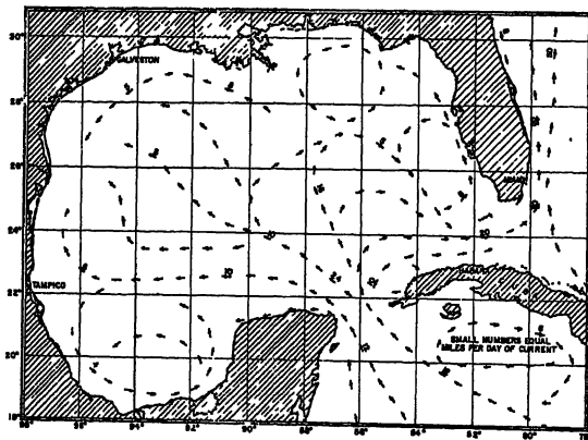
Figure 18 Surface currents in the Gulf of Mexico in December (From Laipper, 1954).
