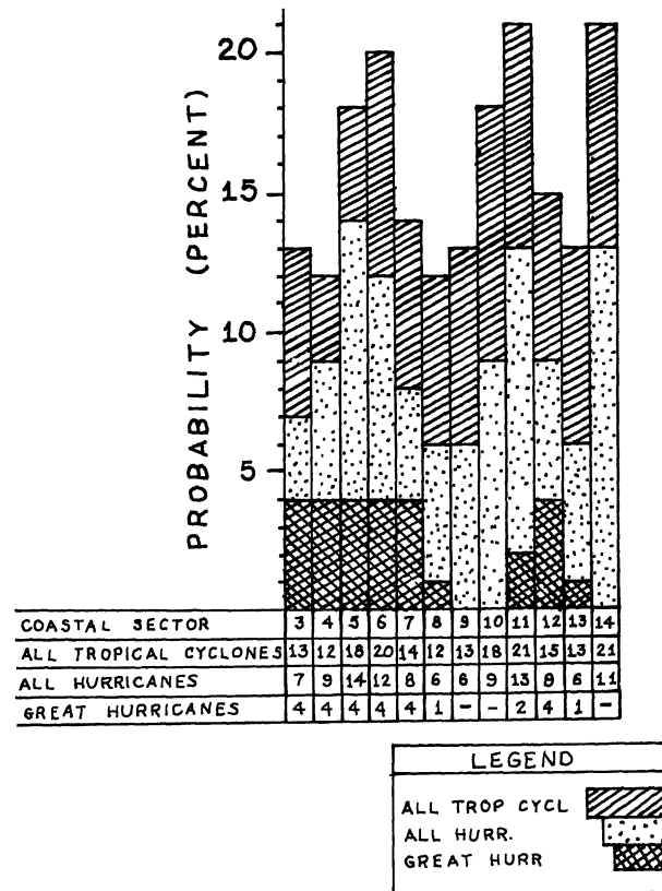
Figure 14. Cyclone probabilities for coastal sectors along the Gulf Coast (From Simpson and Lawrence, 1971). See Figure for location of indicated coastal sectors. The authors used the following groupings of cyclones: All tropical cyclones have winds 40 mph or higher, All hurricanes have winds 74 mph or higher, All great hurricanes have winds 125 mph or higher.
