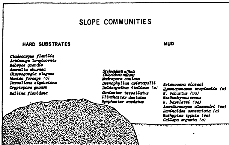
Figure 32. Slope communities. Many species found here are common throughout the Gulf of Mexico and are found in the Atlantic Ocean and the Caribbean Sea. (from Collard and D'Asaro, 1973)
