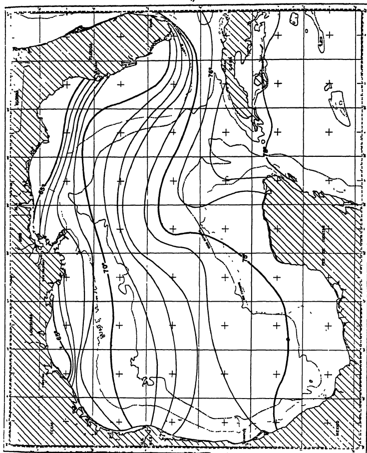
Figure 20. Average sea surface temperatures ( F ) for February. (from Leipper, 1954; after Fuglister, 1947)
