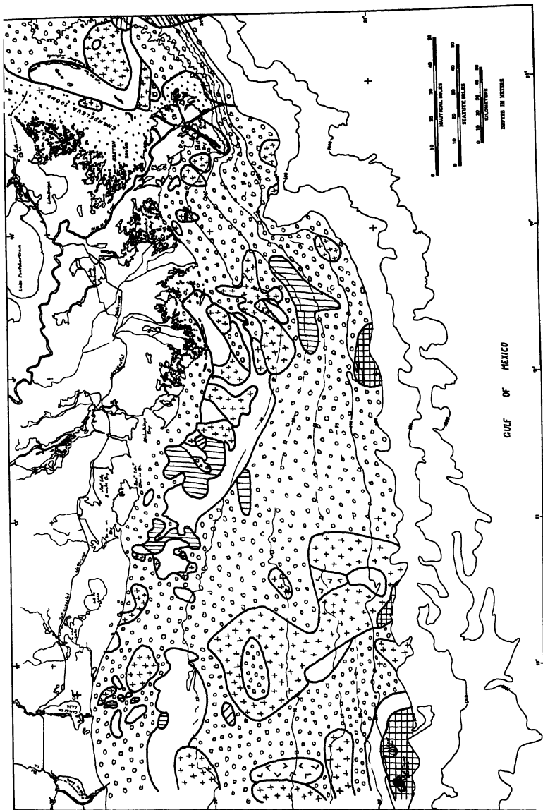
Figure 9. Surface sediment distribution.
