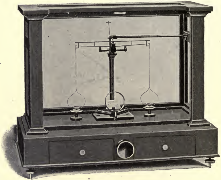
FIG. 26. BUTTON BALANCE.
