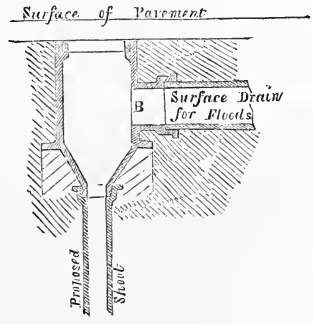
Section in a line with Street.
