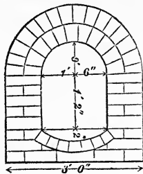
Transverse Section.
