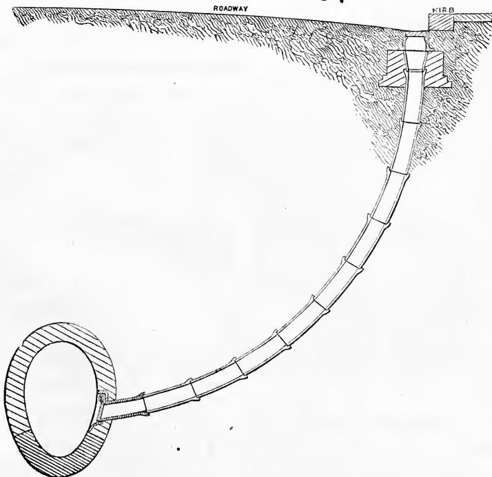
Section of Gully Drain from Grating to Sewer.
