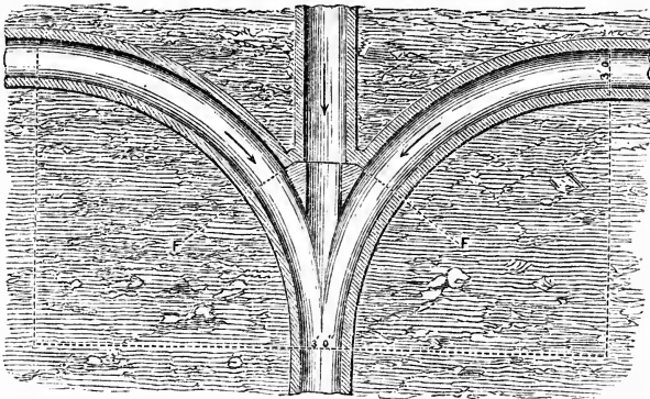
Plan showing the mode of forming the junctions of two side sewers with a leading one.
