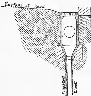
Section across Street.
