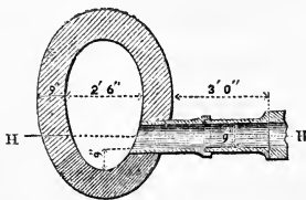
Section showing the mode of connecting drain with sewer.
