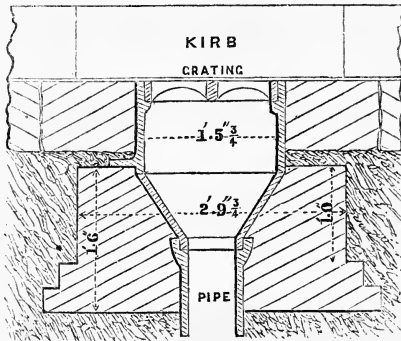
Section of Drain and Flap at Vent.
