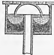
Section of an ordinary Bell-trap, showing deposit of filth,
