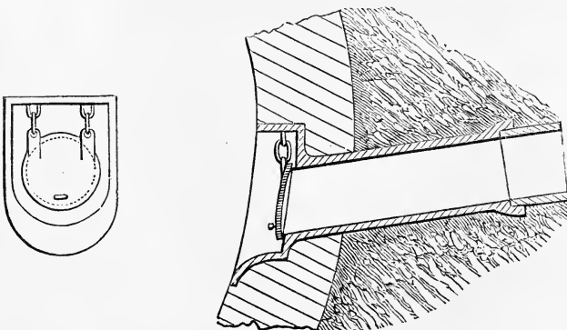
Front View of Flap.
