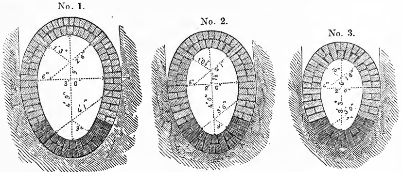
The darker portions of the Inverts to be worked in cement.
