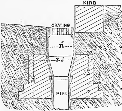
Transverse Section of Gully and Grating on A. B.
