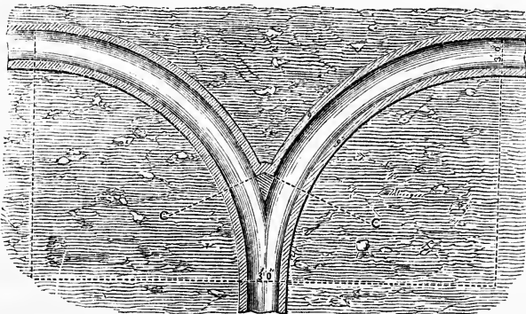
Plan showing the mode of forming the junctions of two side sewers where a straight one terminates.
