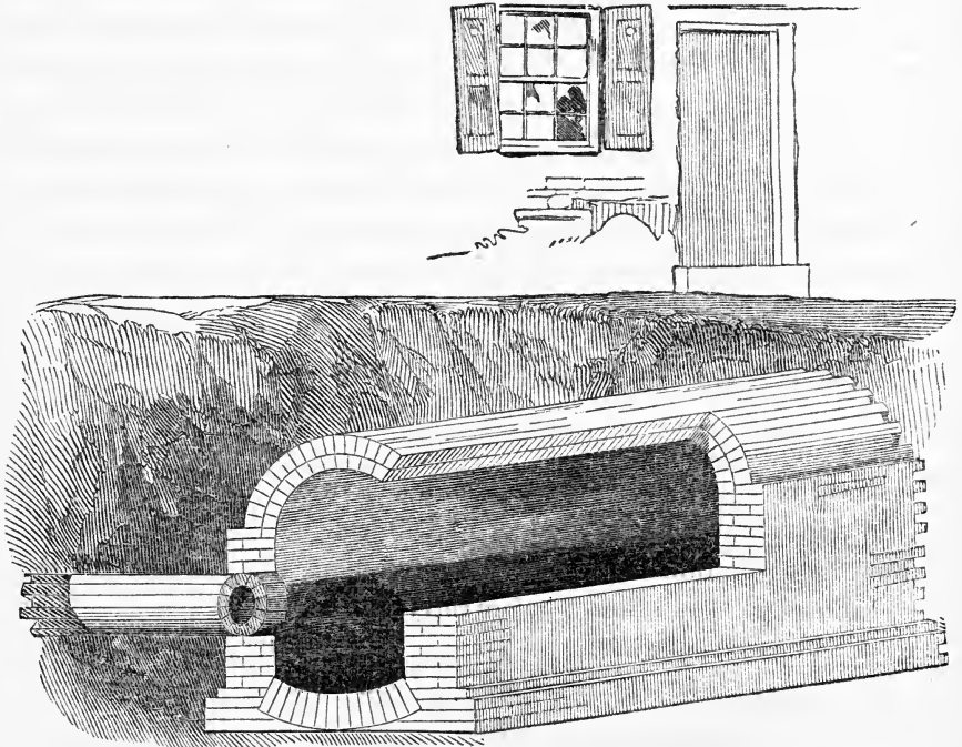
Sewer constructed in Langley Court, Long Acre.
