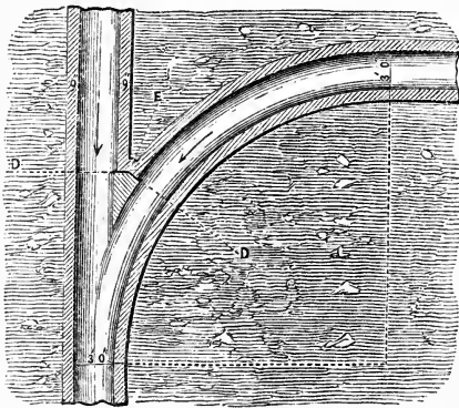
Plan showing the mode of forming the junction of a side sewer with a leading one.
