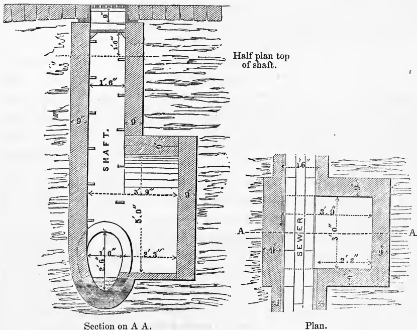
Plan and Section of Shaft. ROADWAY.
