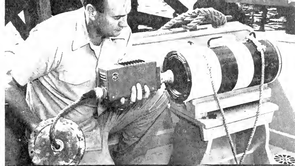
Camera unit, RCA JTV-5, is inserted into watertight housing.
