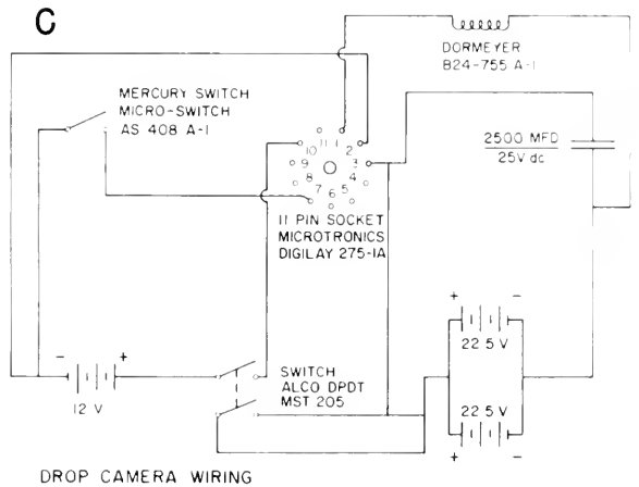
FIGURE 1.—(A) The Isaacs-Brown free vehicle drop camera. (B) A lateral view of the upper camera housing. Once the camera was upright, the mercury switch closed and the electric timer discharged every 24 or 48 s which caused the solenoid to contract bringing the depressor arm down on the shutter release. The strobe light fired simultaneously and the film was advanced automatically. (C) The wiring diagram for the camera system.
