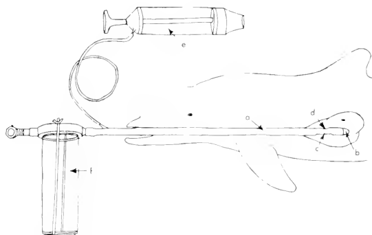
FIGURE 1.—Schematic of lavage device. Entubation tube (a), Nylon end plug (b), side suction port (c), irrigation port (d), irrigating solution hand pump (e), stomach content collection chamber (f).
