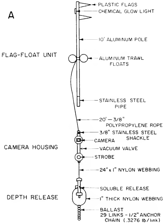
FIGURE 1.—(A) The Isaacs-Brown free vehicle drop camera. (B) A lateral view of the upper camera housing. Once the camera was upright, the mercury switch closed and the electric timer discharged every 24 or 48 s which caused the solenoid to contract bringing the depressor arm down on the shutter release. The strobe light fired simultaneously and the film was advanced automatically. (C) The wiring diagram for the camera system.
