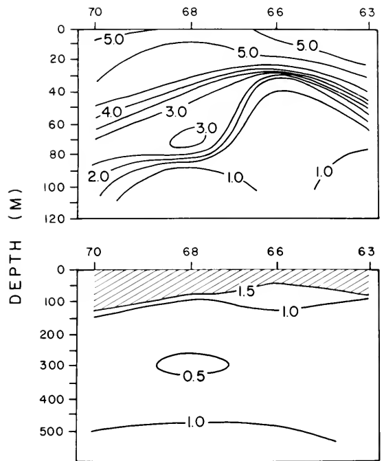
FIGURE 3.—One of the transects of dissolved oxygen concentration (milliliters per liter) produced from Undaunted data (8-16 March 1968). From Cook et al. 1974.
