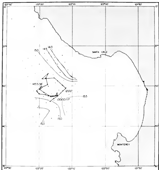
FIGURE 2.—Movements of albacore number 4 as indicated by ultrasonic tracking and contoured field of sea surface temperature in degrees Celsius. Triangles on fish track indicate hourly position. The time and date that tracking commenced is noted at the starting location and shown above and below a slash mark, respectively. The 0000 and 1200 h local time positions are also indicated. Dots show where temperature observations were made by David Starr Jordan . Temperatures below 15.0°C are shaded.
