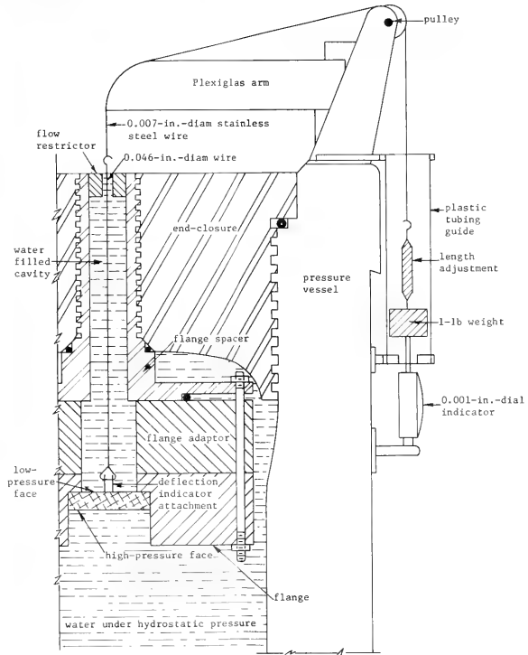
Figure 4e. Schematic drawing of deflection measuring apparatus and flange mounting used in the testing of windows.
