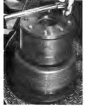
Figure 4c. Torquing down the retaining ring.
