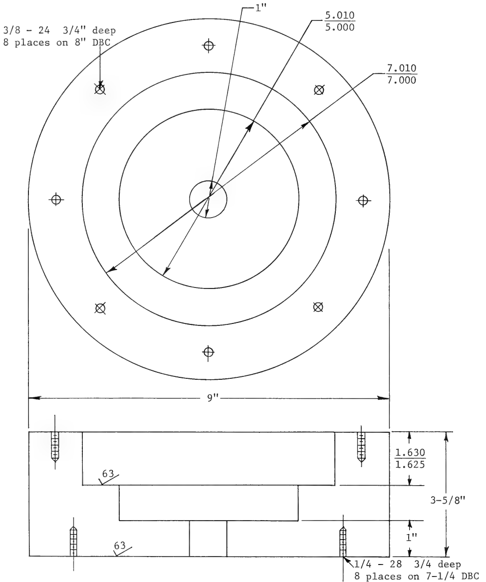
Figure 2a. Dimensions of window seat and opening diameter in the test flange for the 7-inch diameter EDU window, the seat and opening in the test flange are the same as in the EDU chamber window flanges.
